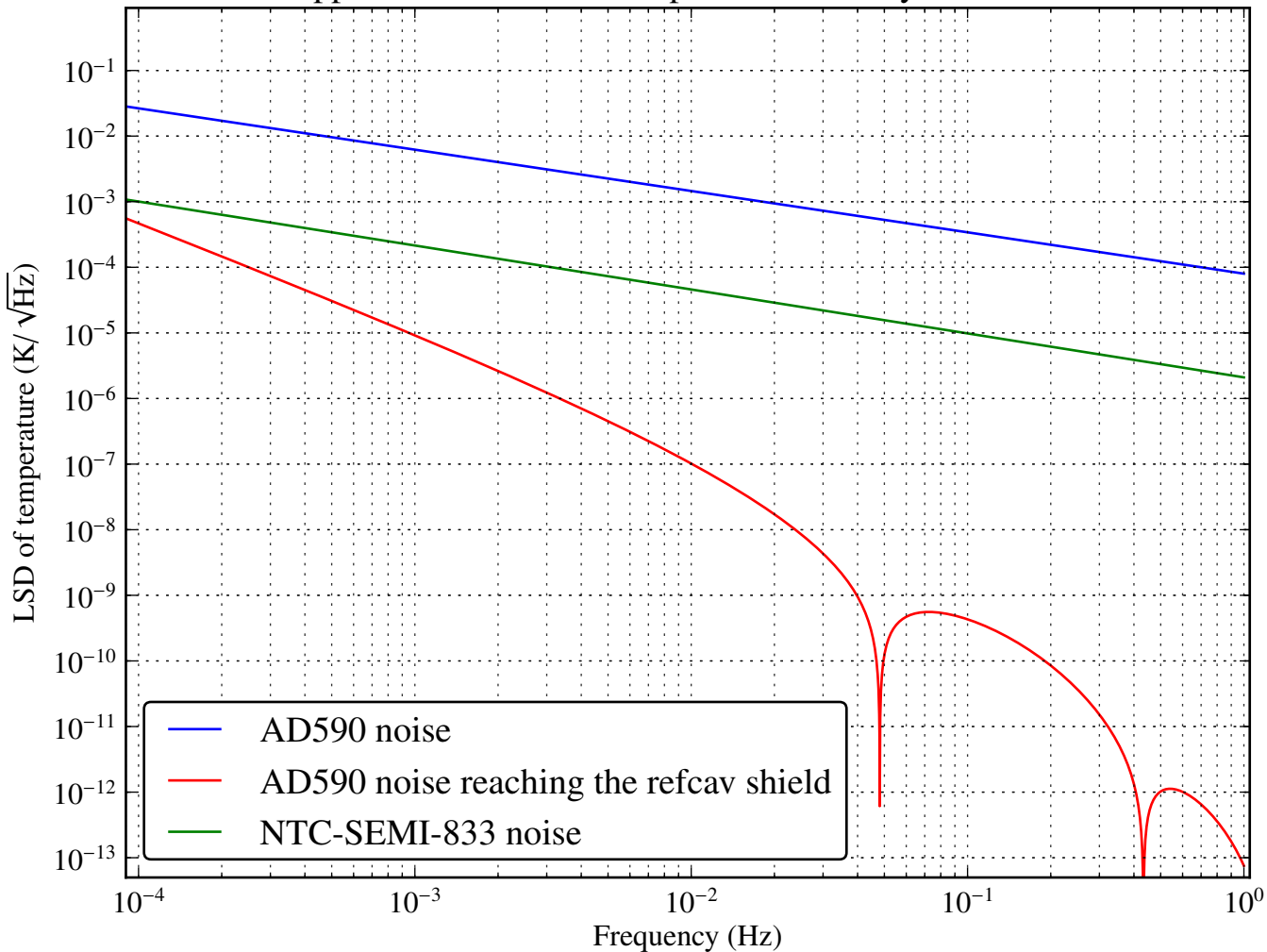
Suppression of AD590 temperature noise by vacuum can
