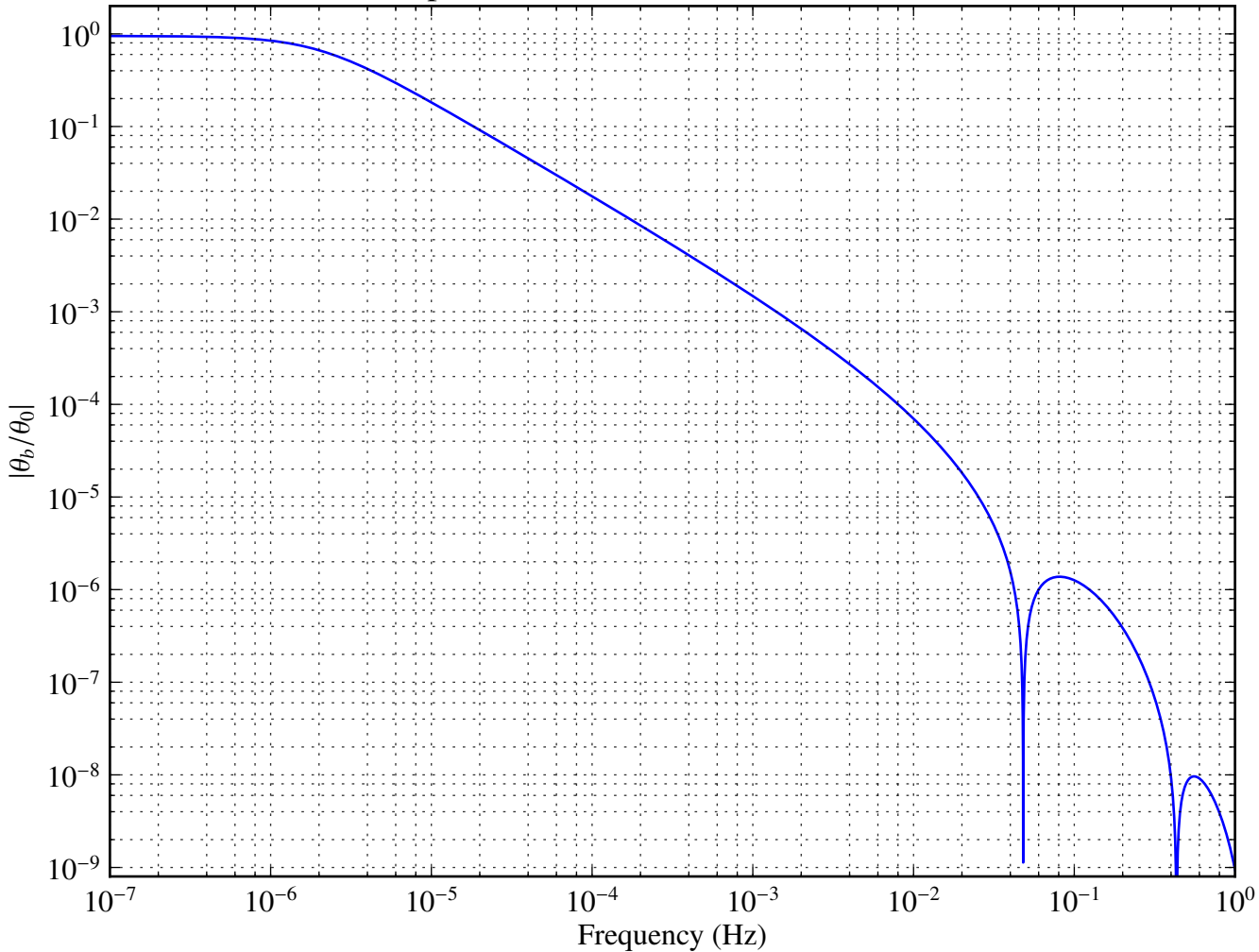
Transfer function of temperature fluctuations from outer surface to radiation shield
