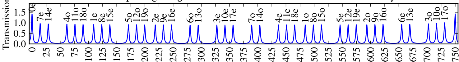
Mode spacing for g = 0.637 and L = 0.2 m for a 3-mirror cavity
