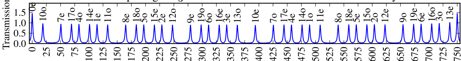
Mode spacing for g = 0.610 and L = 0.2 m for a 3-mirror cavity
