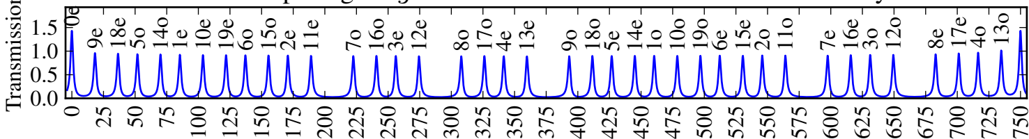
Mode spacing for g = 0.775 and L = 0.2 m for a 3-mirror cavity
