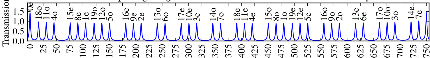
Mode spacing for g = 0.755 and L = 0.2 m for a 3-mirror cavity
