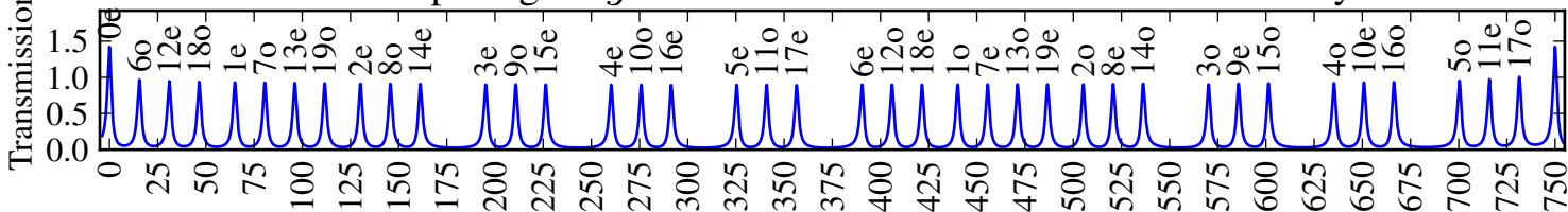
Mode spacing for g = 0.910 and L = 0.2 m for a 3-mirror cavity
