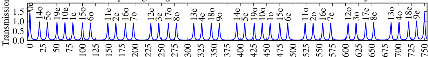
Mode spacing for g = 0.855 and L = 0.2 m for a 3-mirror cavity
