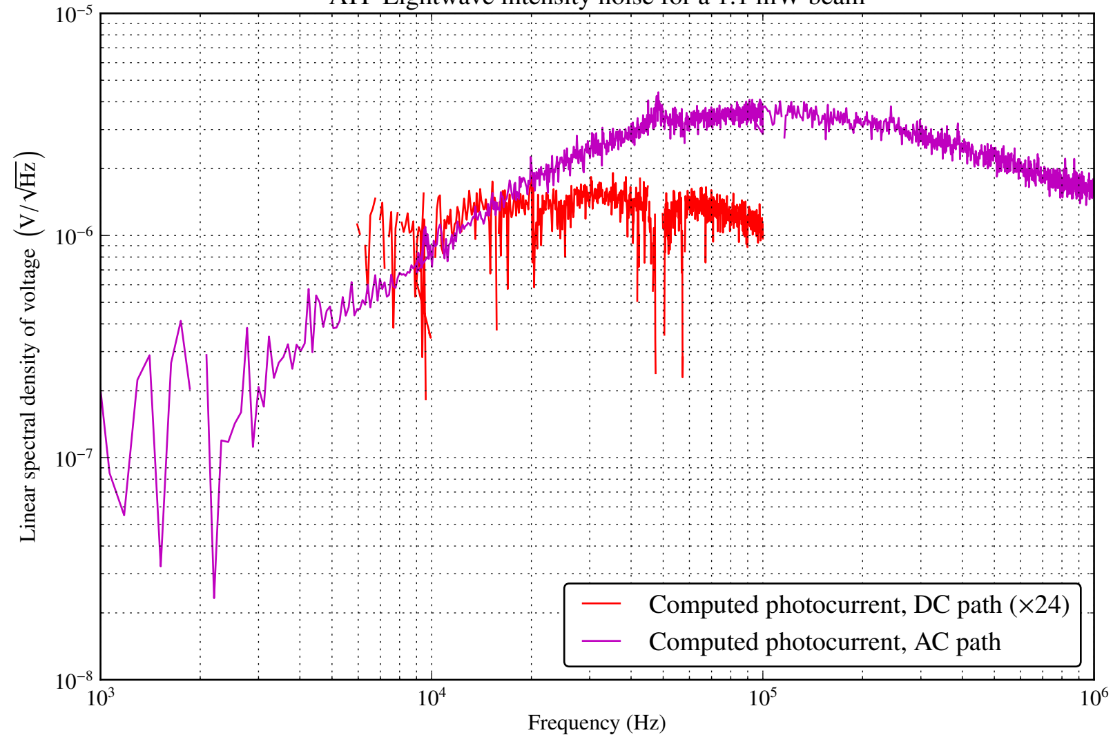
ATF Lightwave intensity noise for a 1.1 mW beam
