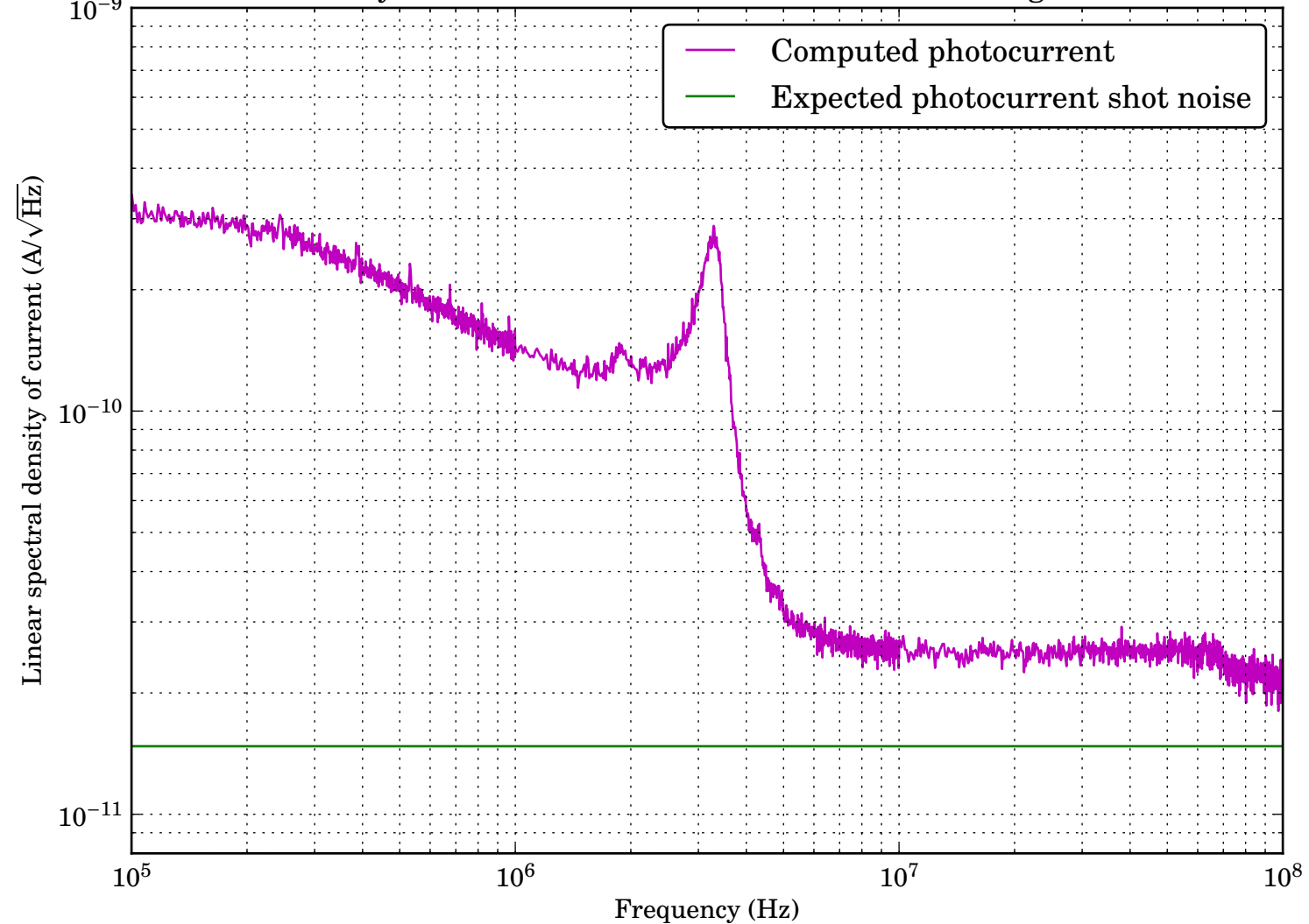
Intensity noise from a 1.0 mW beam from the ATF Lightwave
