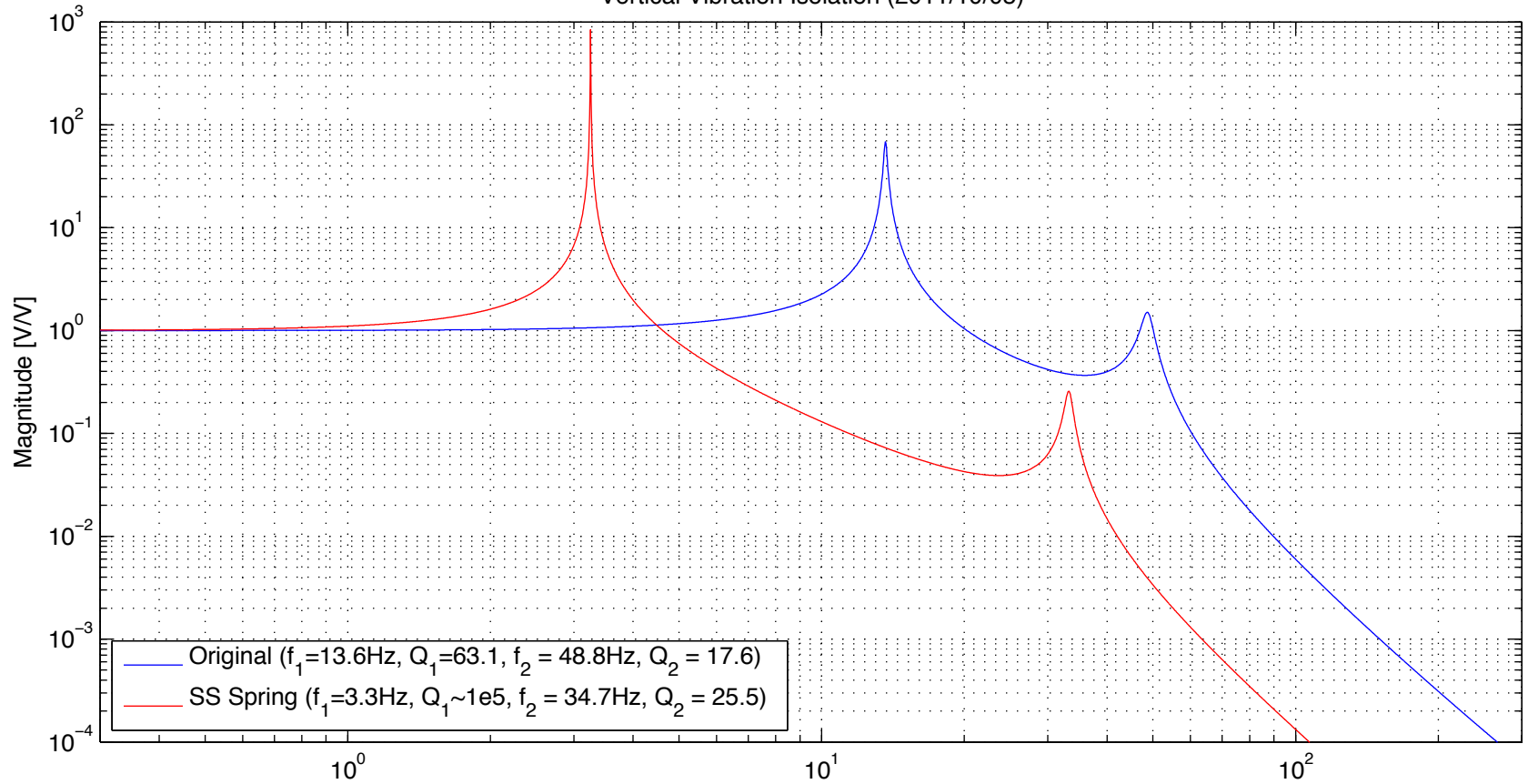
Vertical Vibration Isolation (2011/10/05)
