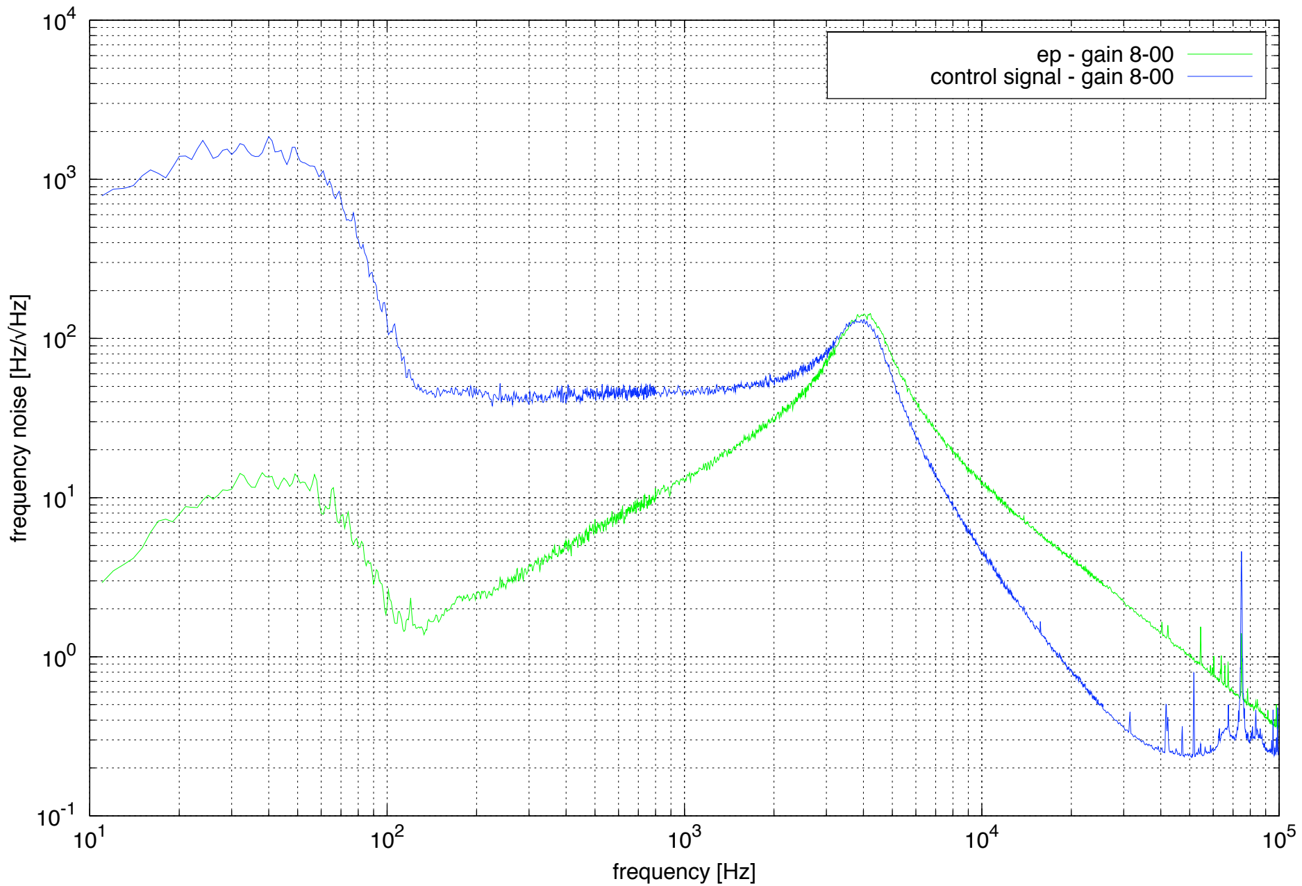
refcav noise - first quick measurement 01/27/2010
