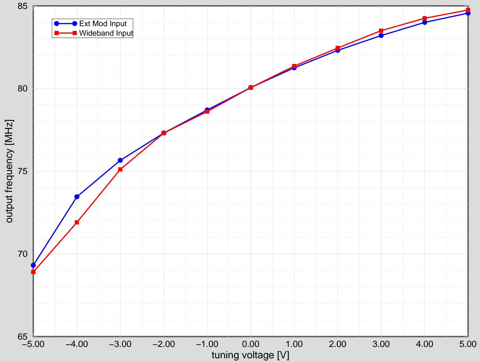
80 MHz VCO D980401-B1-C S/N BL2003 output frequency vs. tuning voltage
