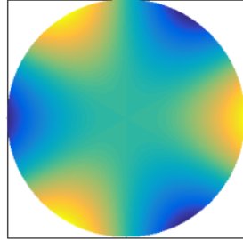
Mode 2, 1664.5 Hz
