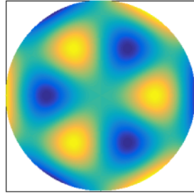
Mode 7, 6775.5 Hz
