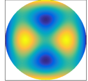
Mode 5, 4416.5 Hz
