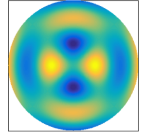
Mode 10, 10238.5 Hz
