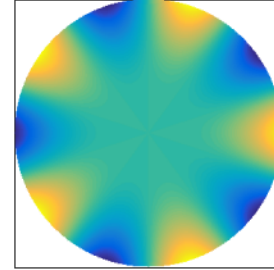
Mode 4, 3890.5 Hz
