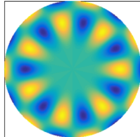
Mode 18, 20300.5 Hz
