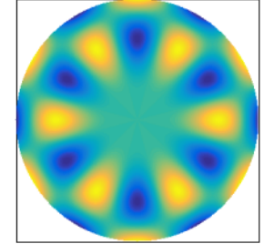
Mode 15, 16279.5 Hz
