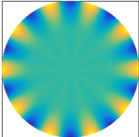
Mode 16, 16768.5 Hz
