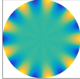
Mode 13, 14240.5 Hz
