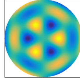
Mode 14, 16165.5 Hz
