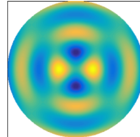
Mode 19, 21498.5 Hz
