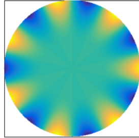
Mode 8, 7313.5 Hz
