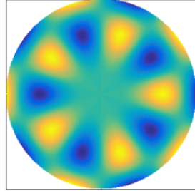
Mode 12, 12676.5 Hz
