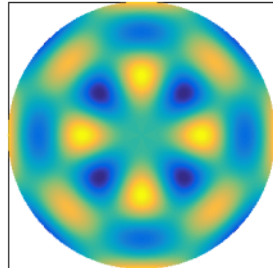
Mode 17, 18760.5 Hz
