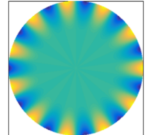
Mode 20, 22761.5 Hz
