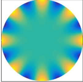
Mode 11, 11424.5 Hz
