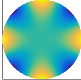
Mode 3, 2533.5 Hz
