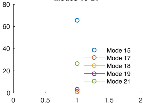
Modes 15-21
