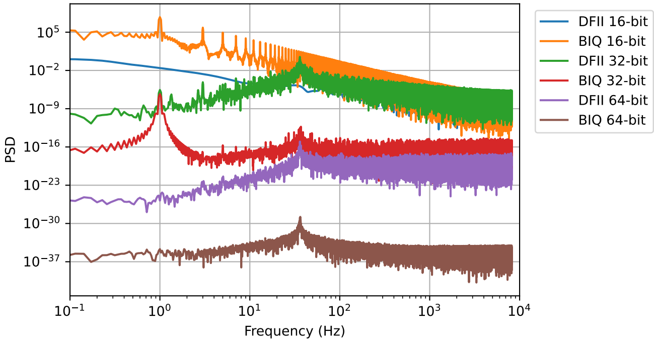
PSD of Quantization Noise for Dual-Sine Input
