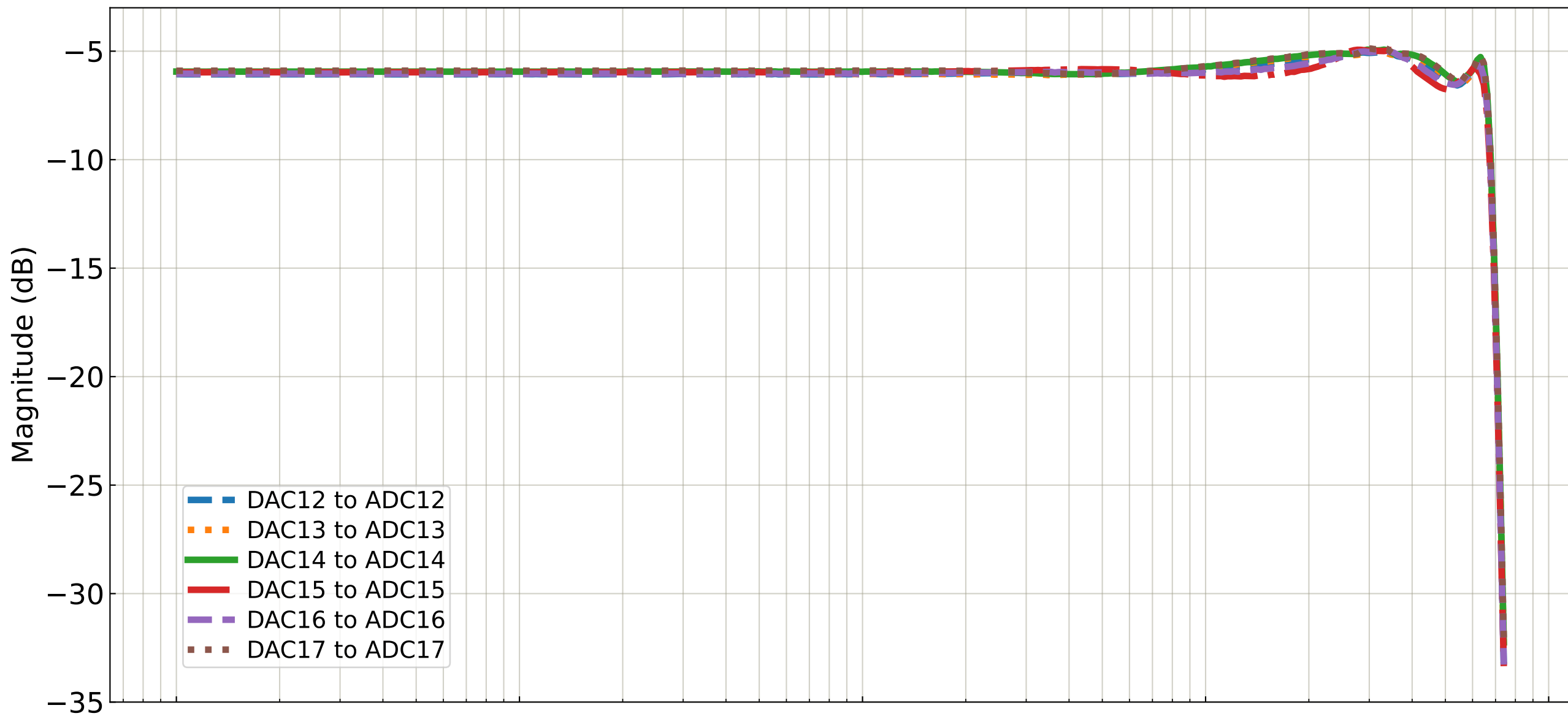
Transfer Function DAC to ADC Test
