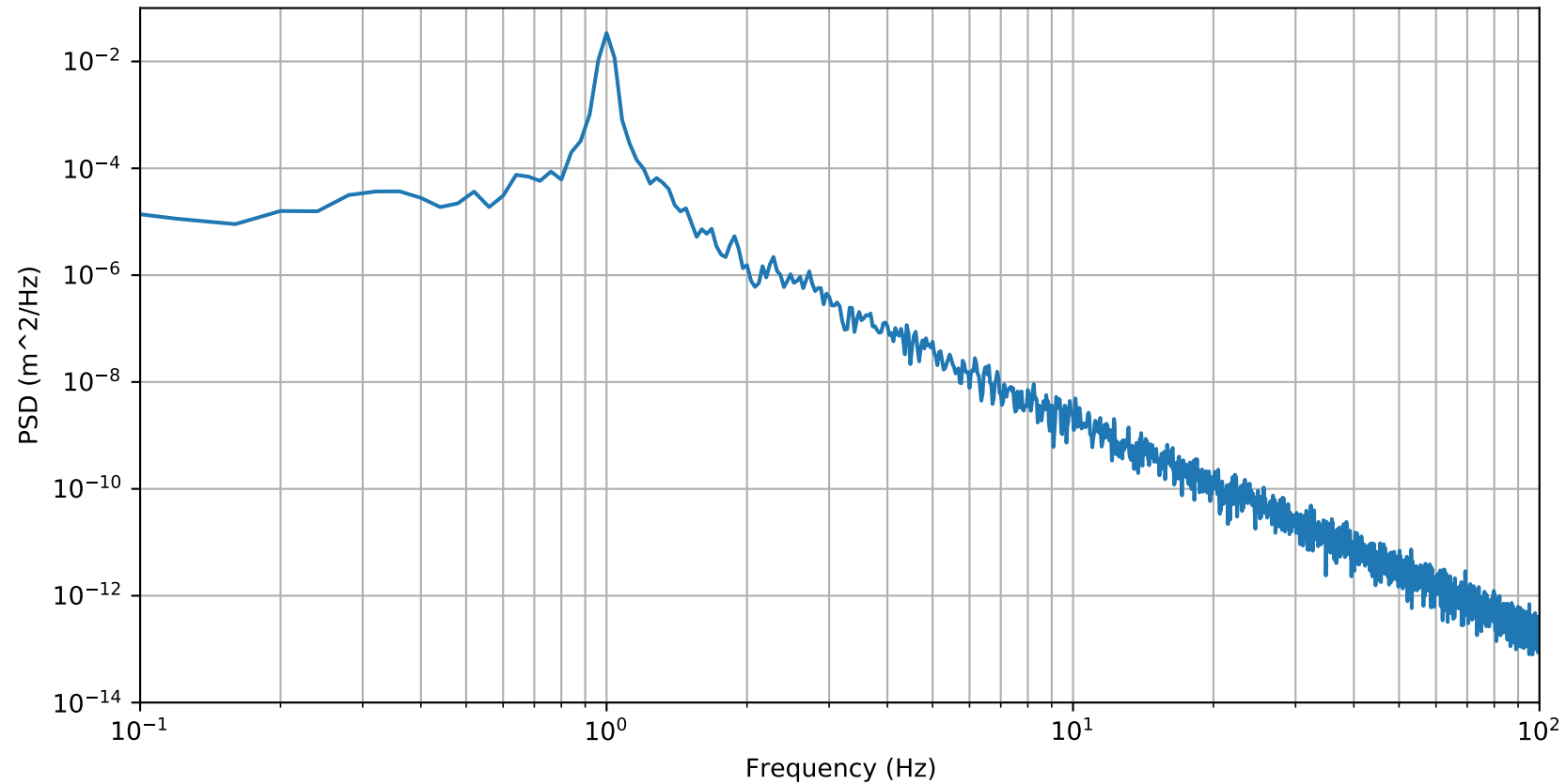
IIR 64-bit Noise Spectrum
