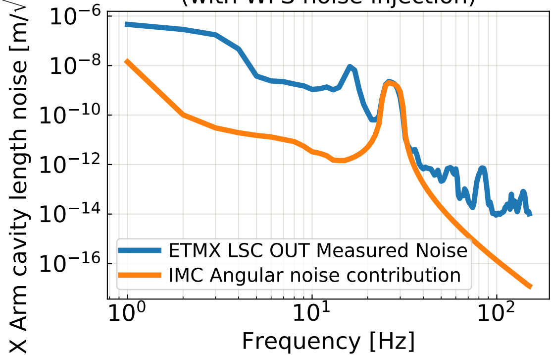
X Arm cavity length noise contributions (with WFS noise injection)
