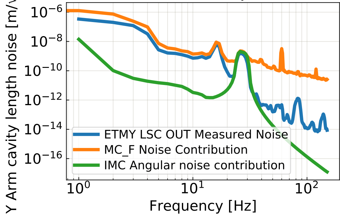
Y Arm cavity length noise contributions (with WFS noise injection)
