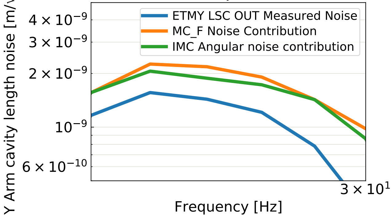
Y Arm cavity length noise contributions (with WFS noise injection) Zoomed In
