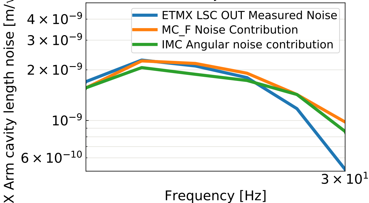
X Arm cavity length noise contributions (with WFS noise injection) Zoomed In
