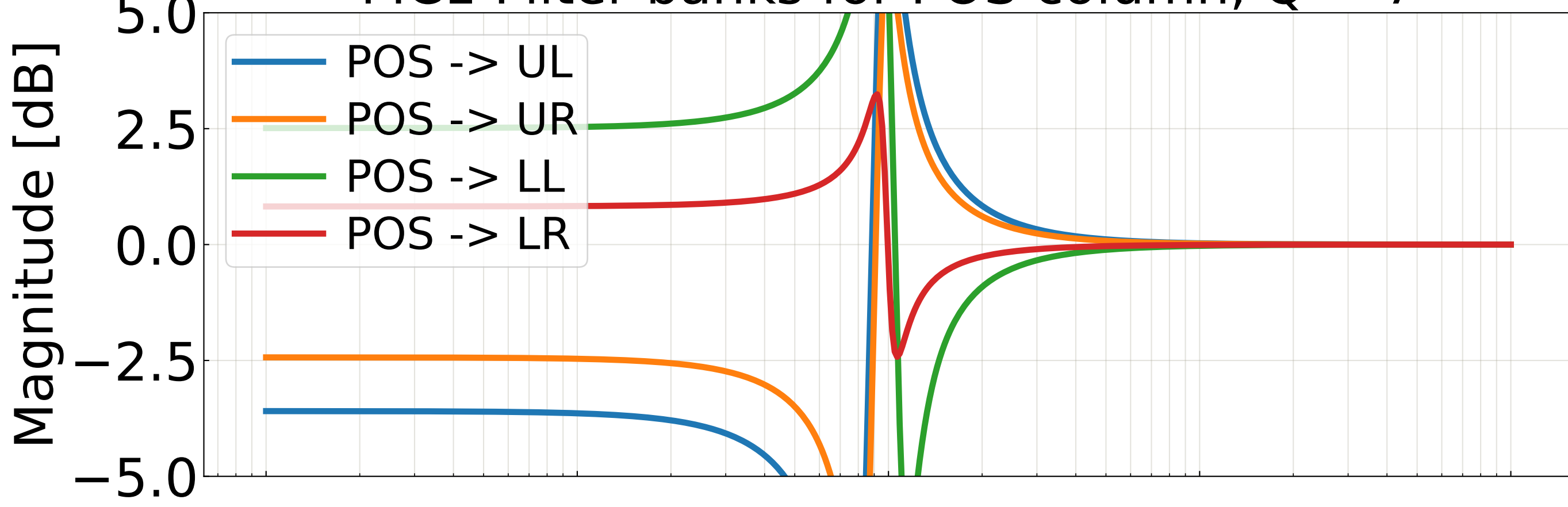
MC1 Filter banks for POS column, Q = 7
