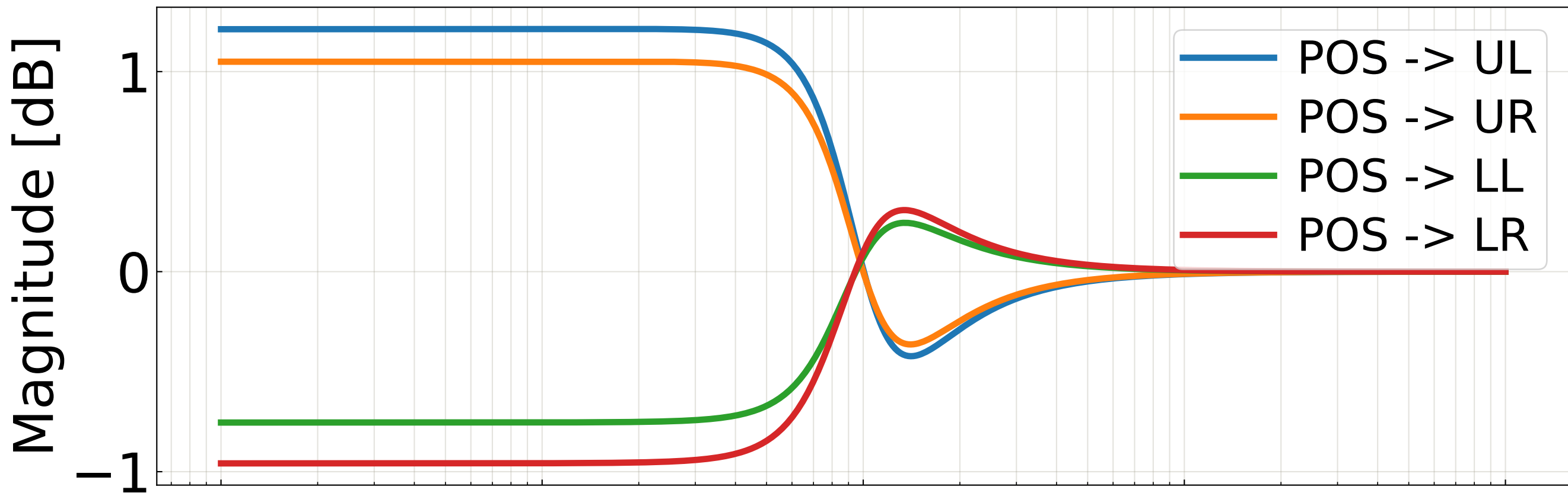
MC2Filter banks for POS column
