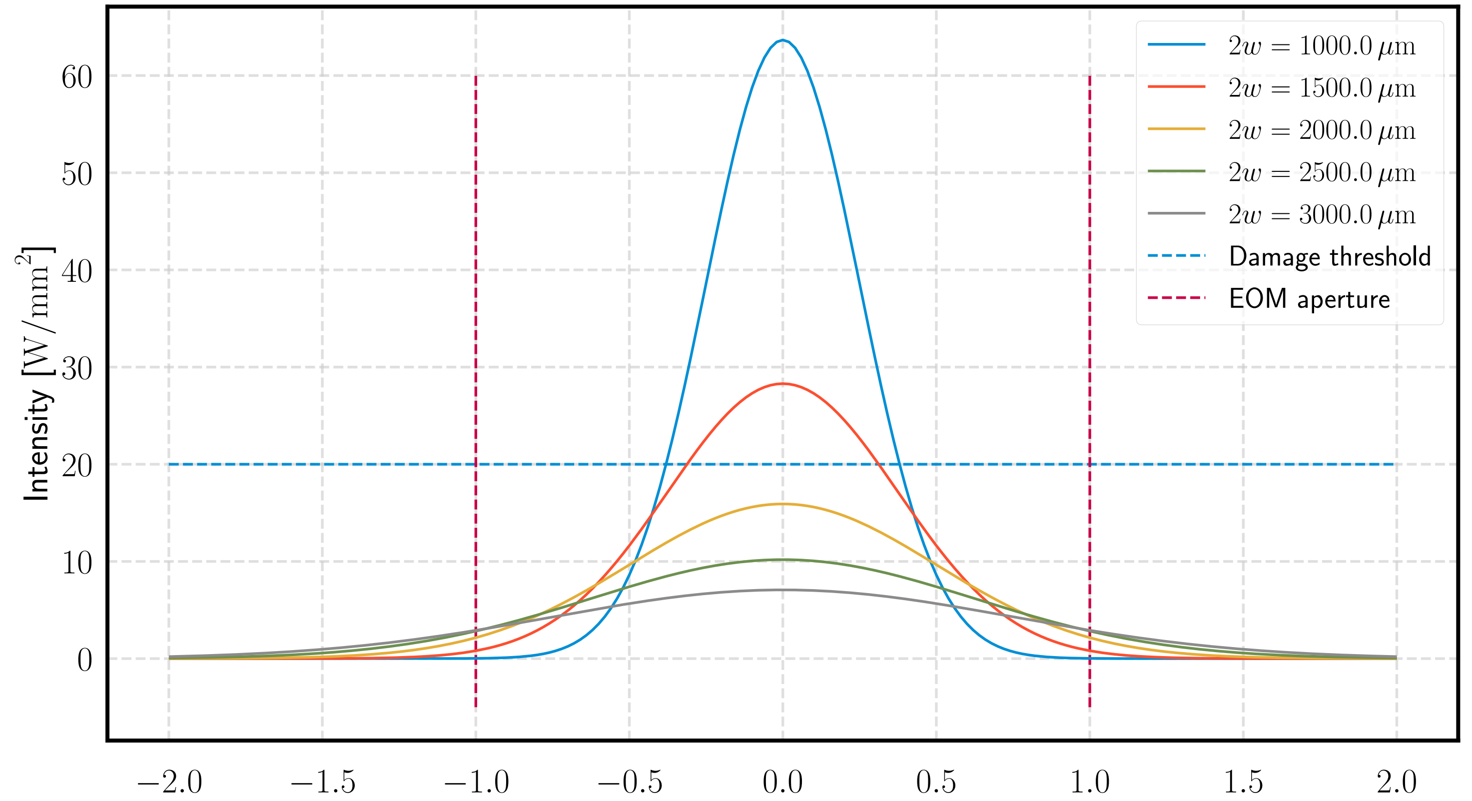
Intensity profiles of a 25 W Gaussian beam
