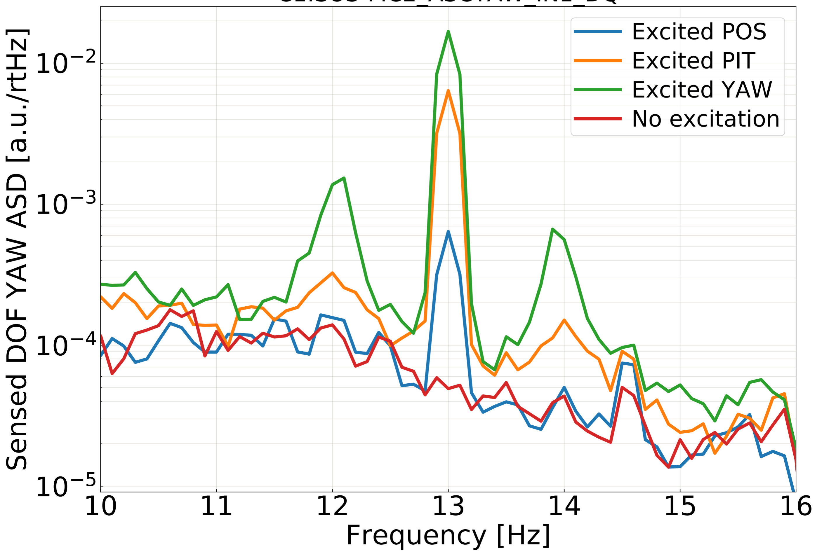
C1:SUS-MC2_ASCYAW_IN1_DQ
