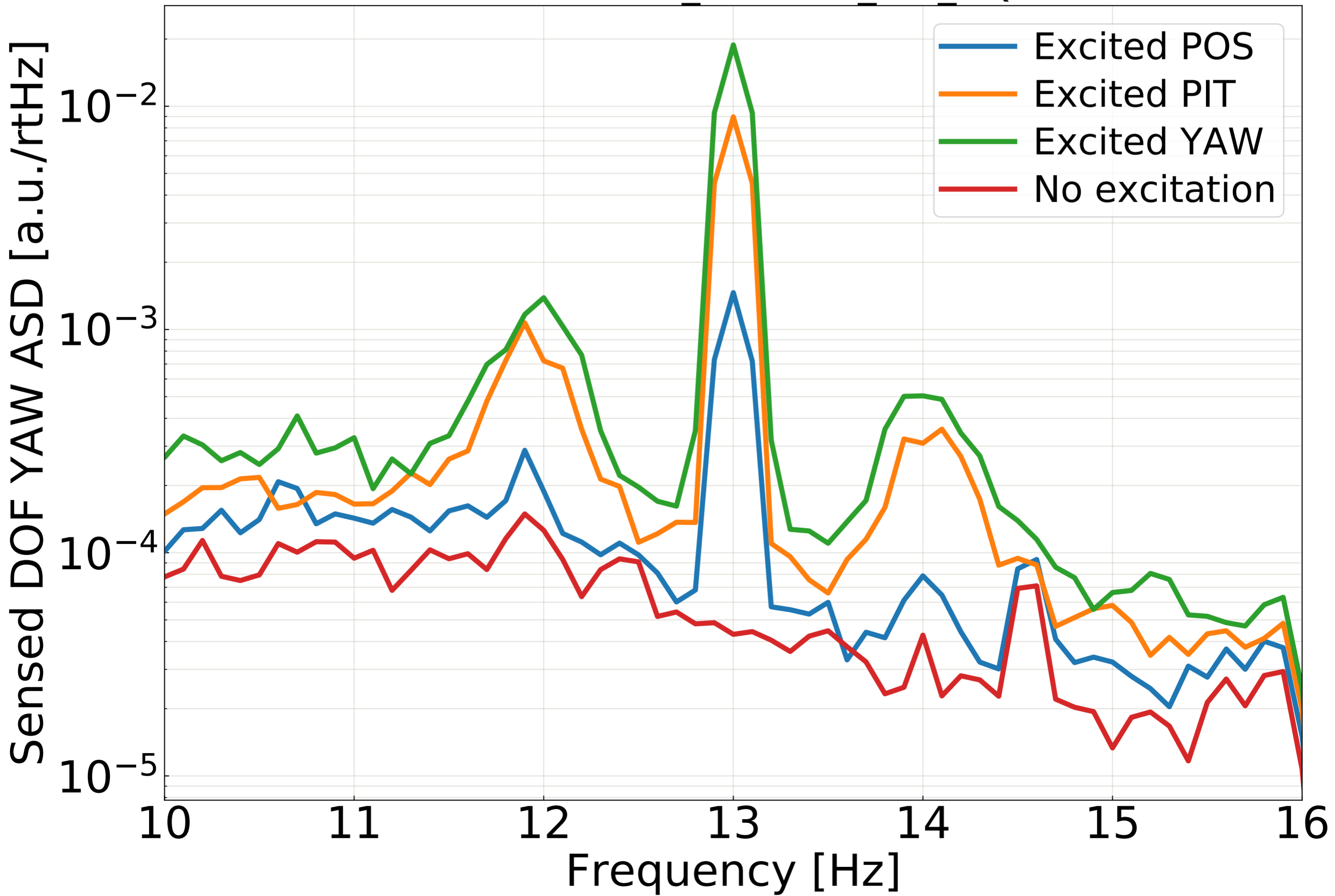
C1:SUS-MC2_ASCYAW_IN1_DQ
