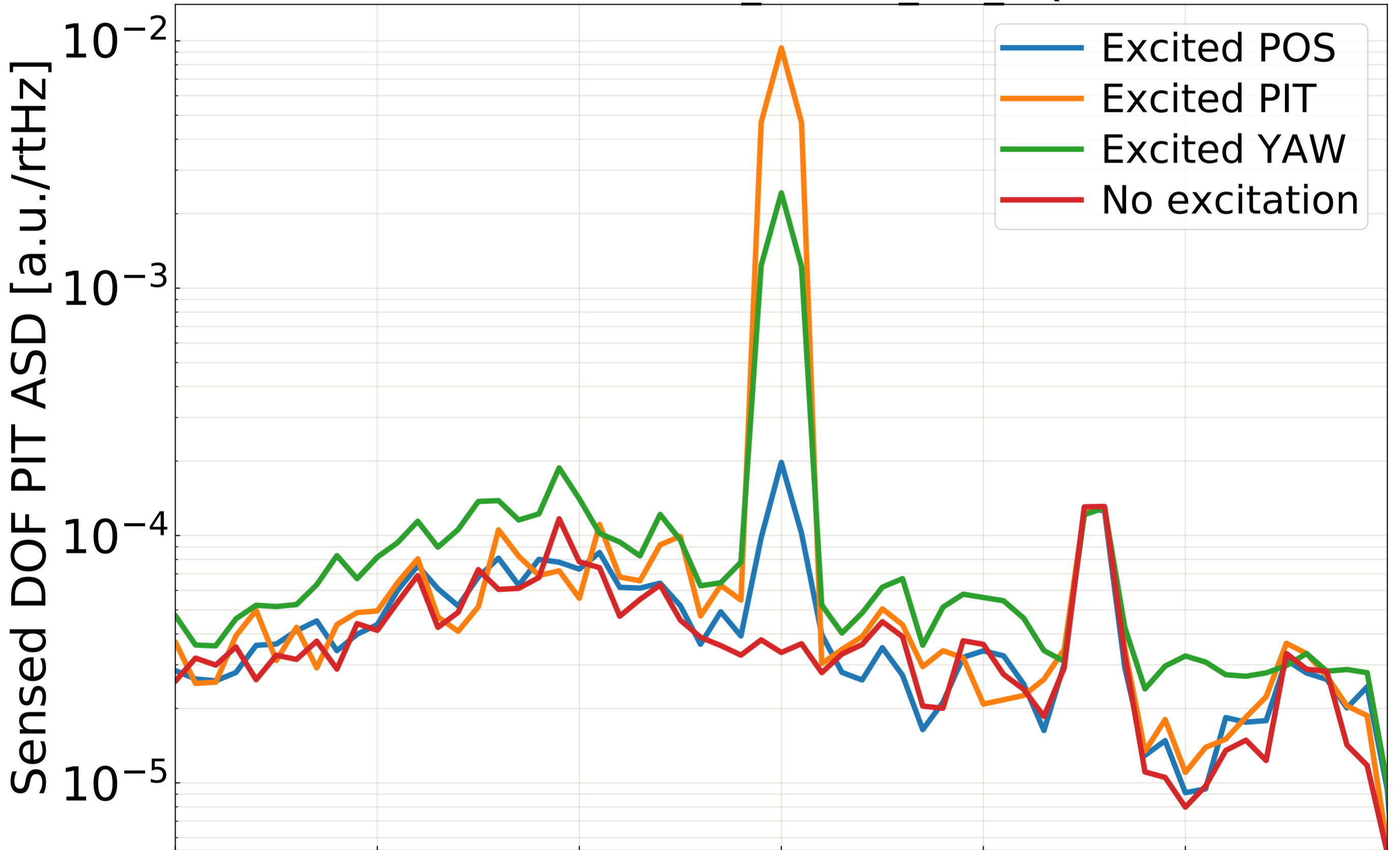
C1:SUS-MC2_ASCPIT_IN1_DQ
