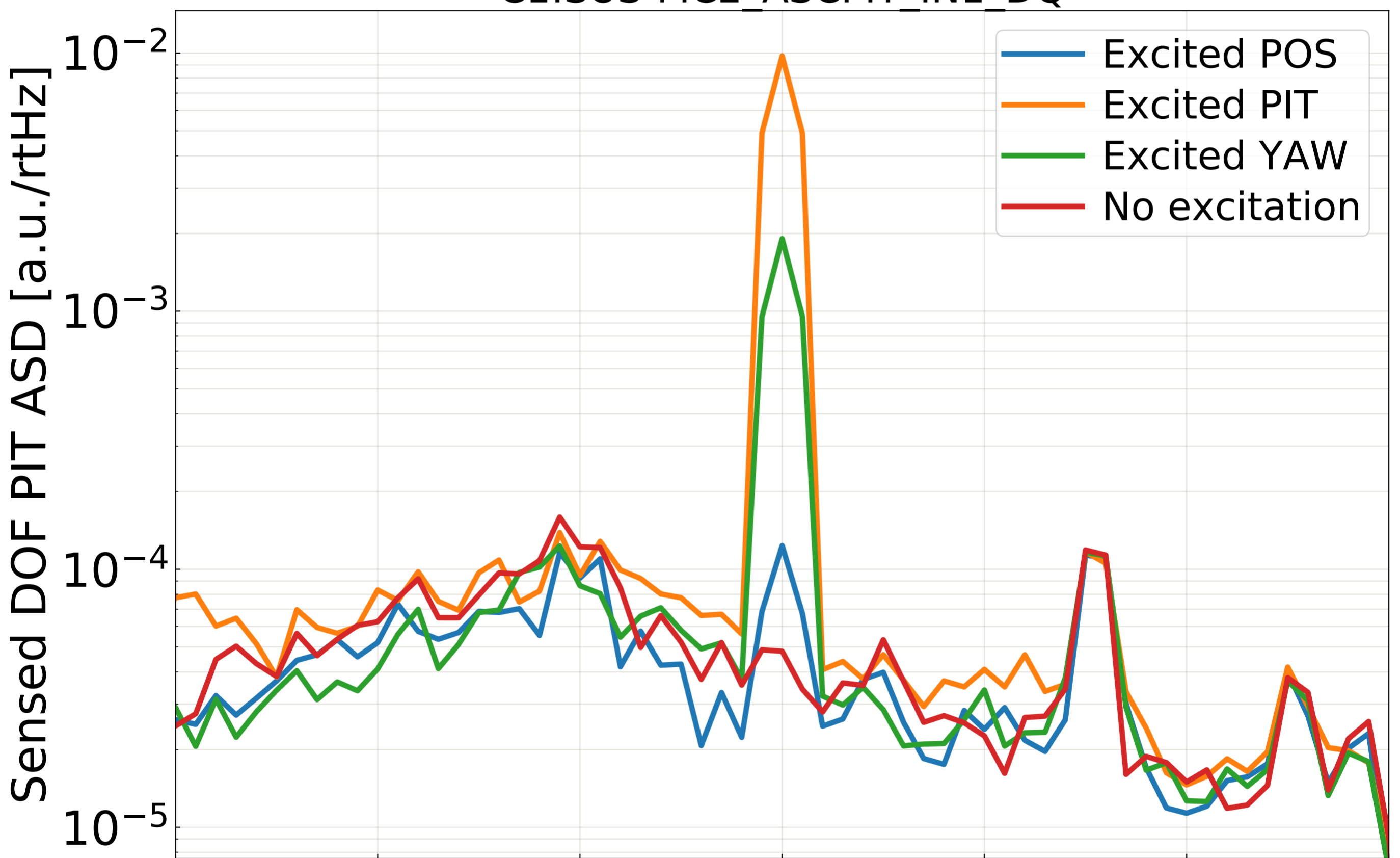
C1:SUS-MC2_ASCPIT_IN1_DQ
