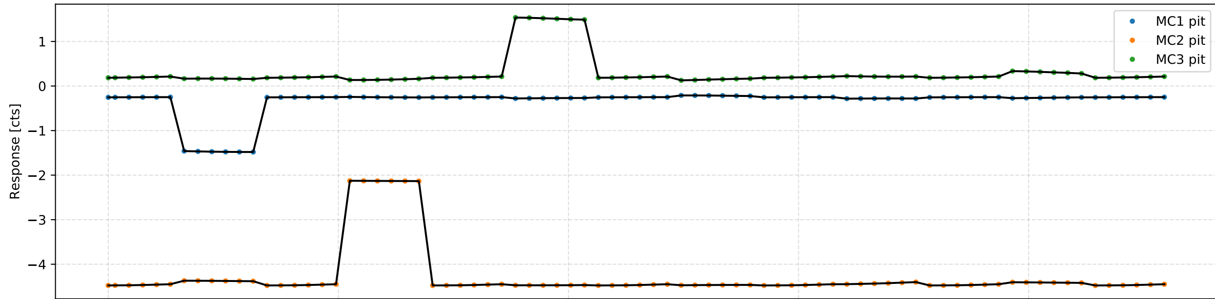
Demodulated MCL response to mirror pitch step, 10\% coil imbalance
