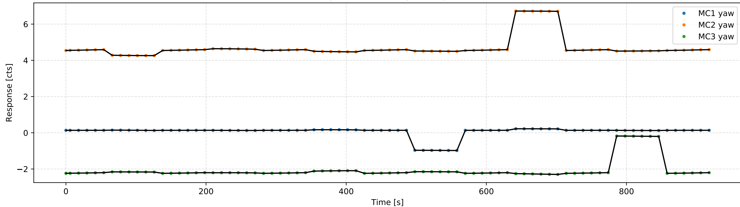
Demodulated MCL response to mirror yaw step, 10\% coil imbalance
