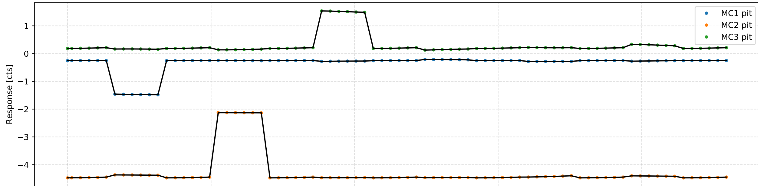
Demodulated MCL response to mirror pitch step
