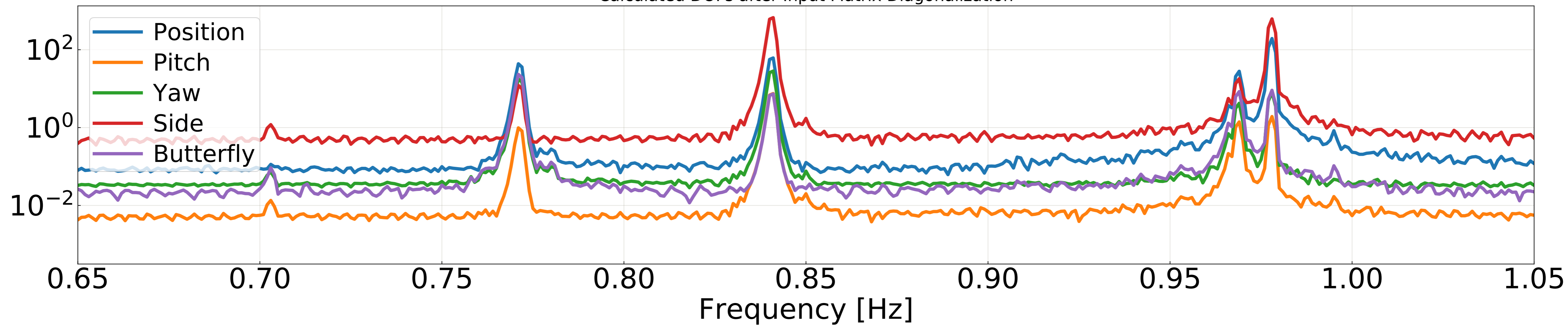
Calculated DOFs after Input Matrix Diagonalization
