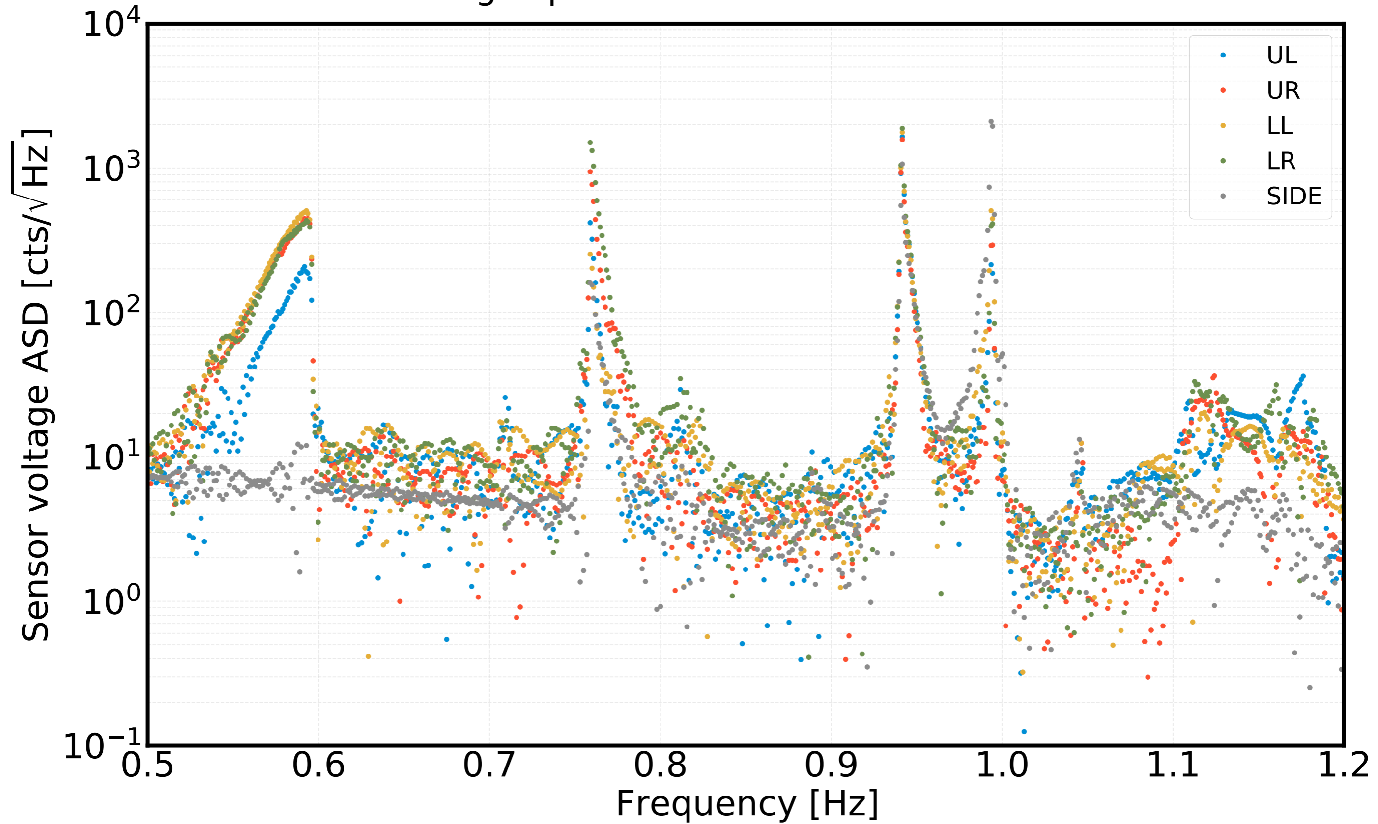
PRM Sensor voltage spectra from 1299355951 for 1024 seconds
