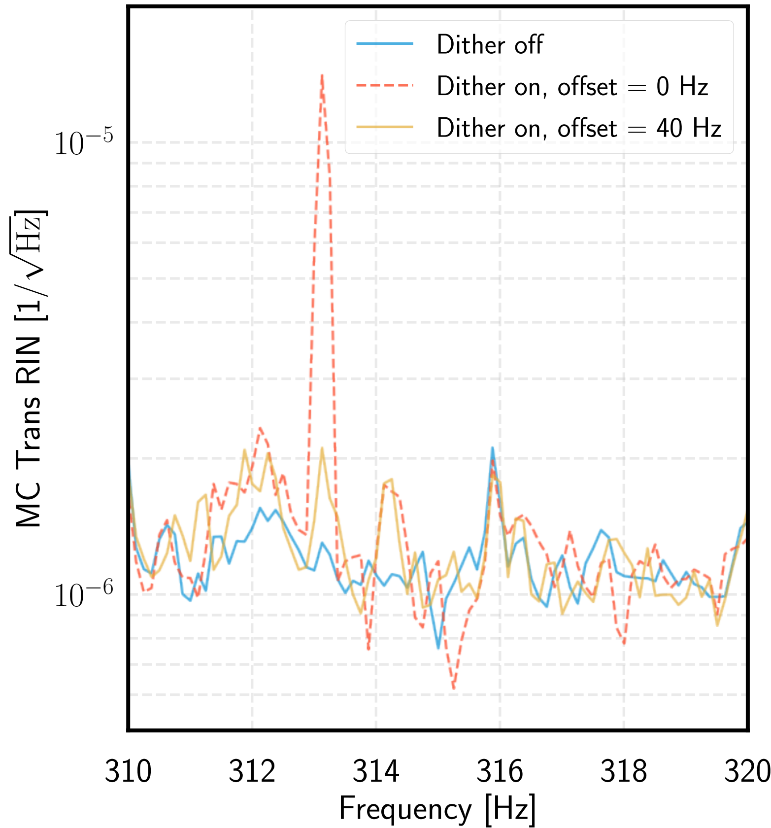
Nulling IMC error point offset
