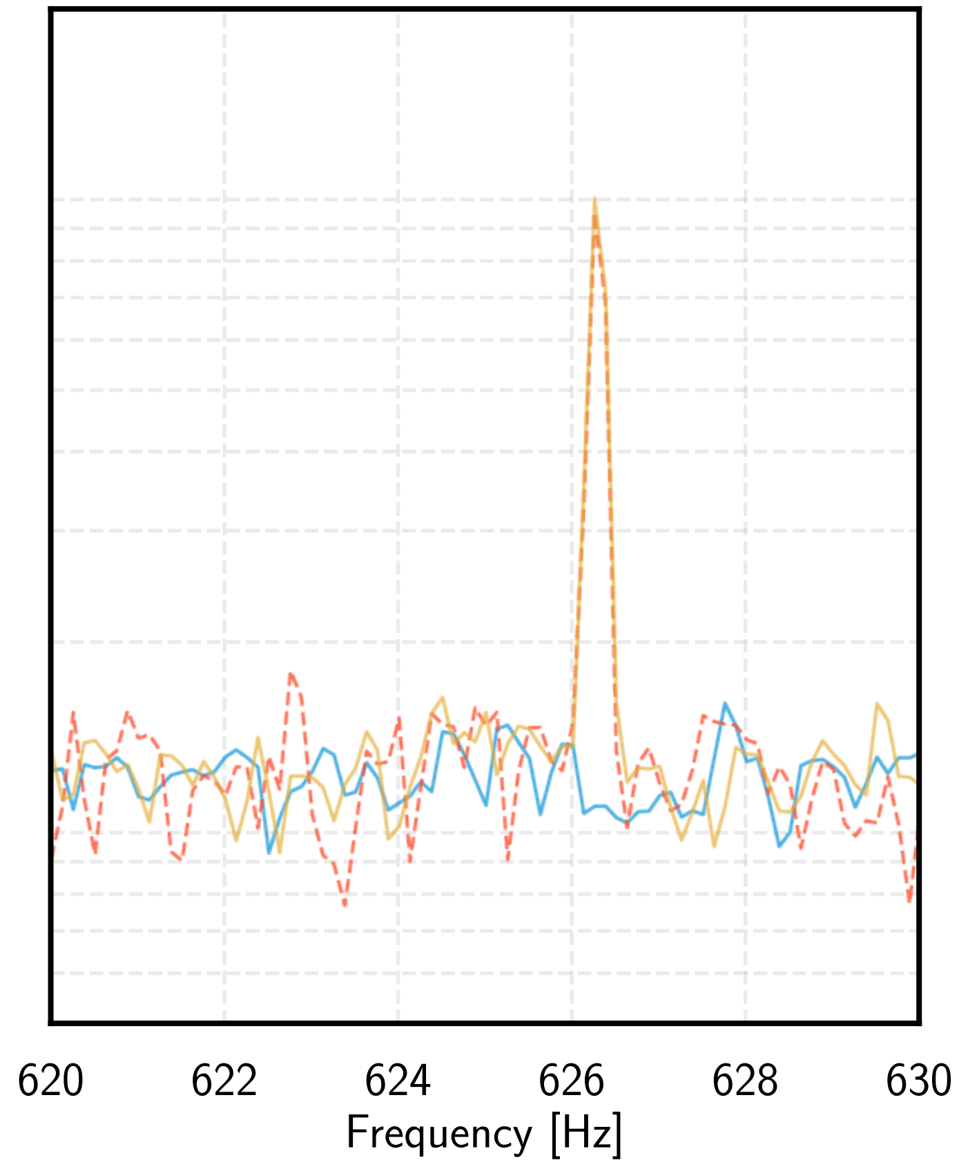
Nulling IMC error point offset
