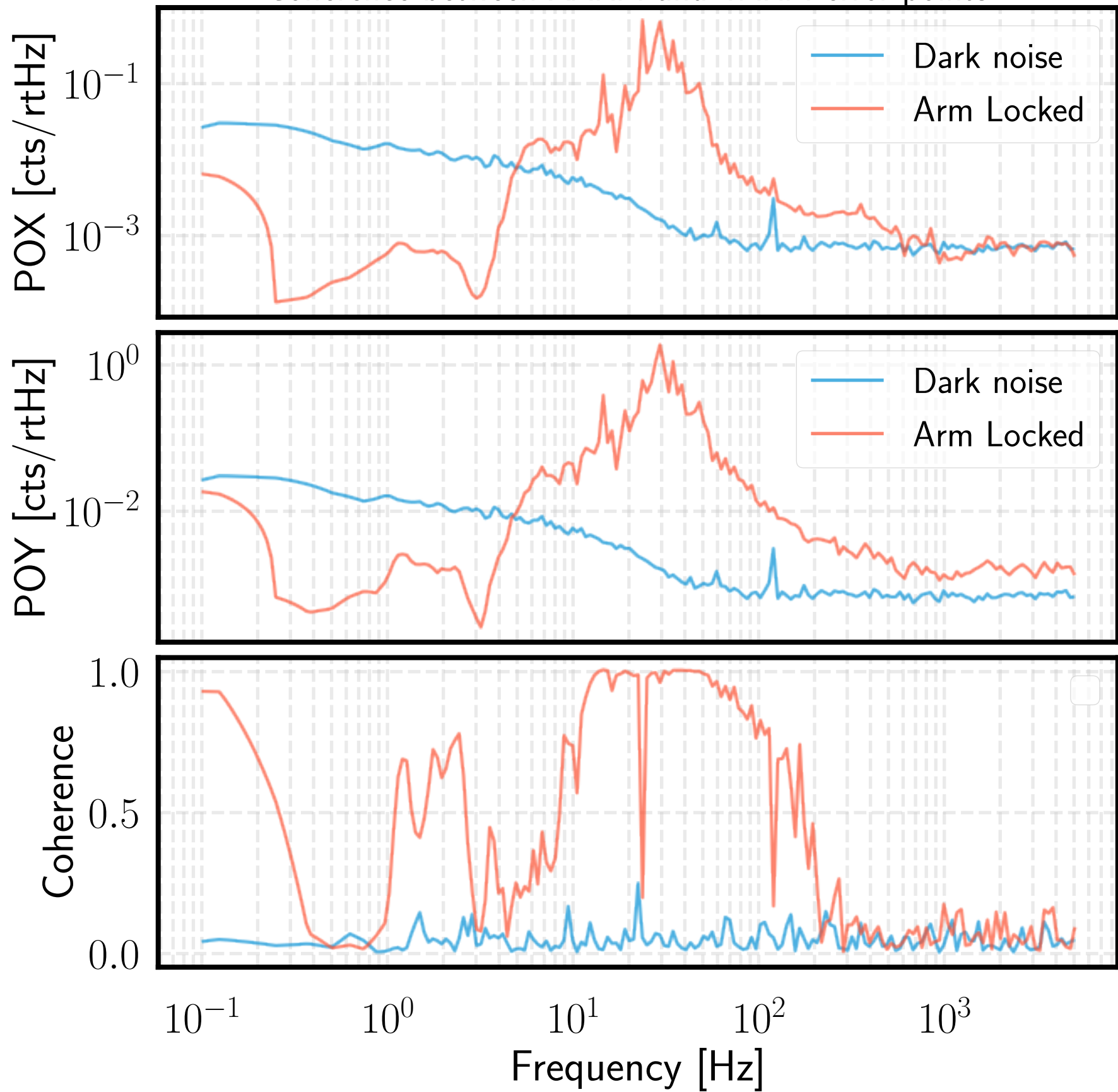
Coherence between XARM and YARM error points
