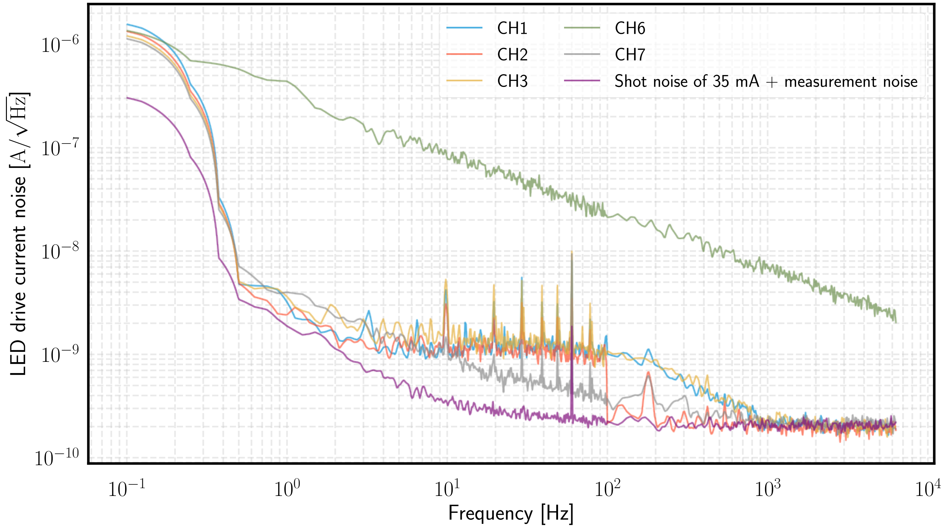
LED drive current noise measured at TP3
