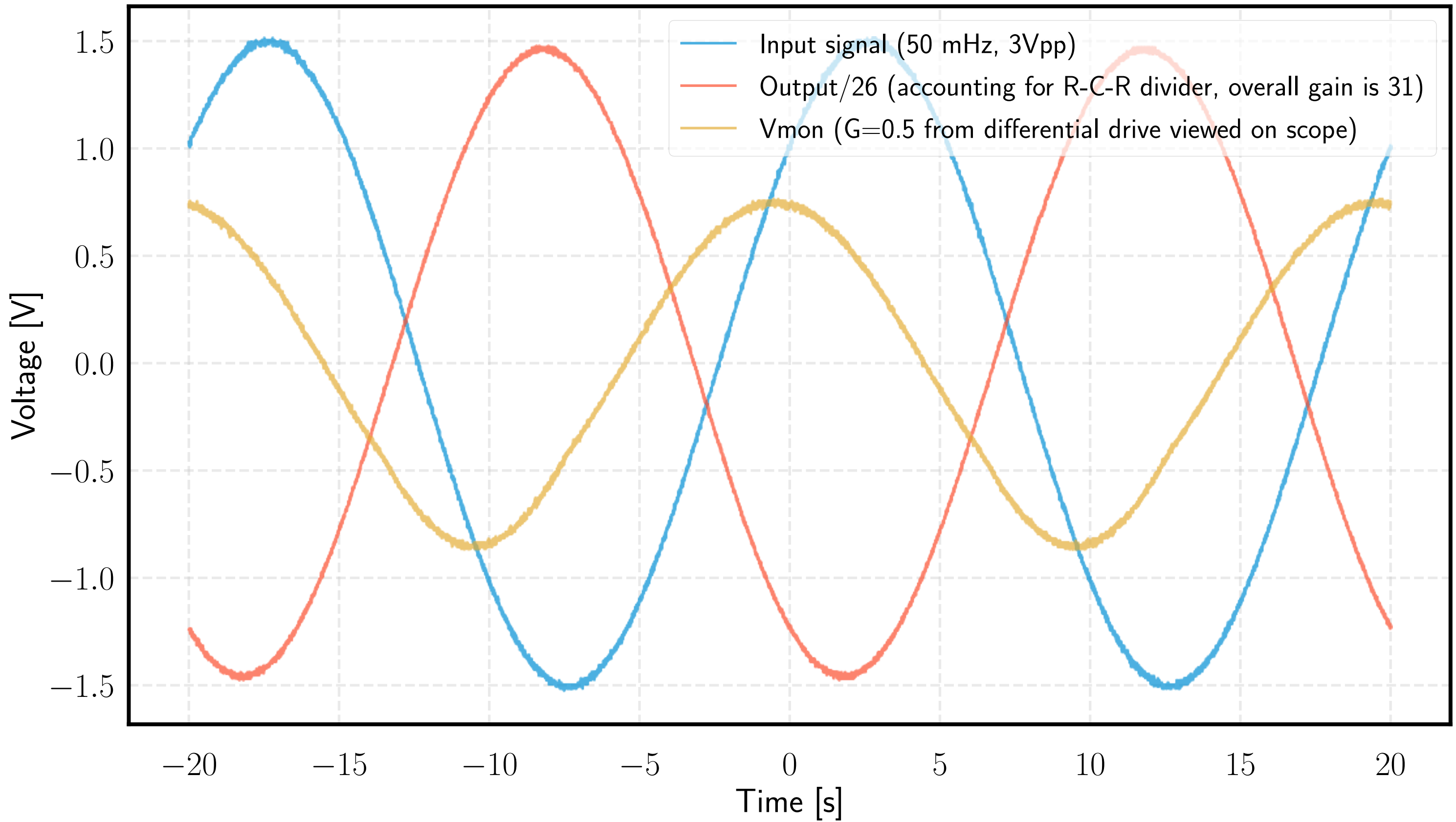
Low frequency time domain test of High Voltage coil driver
