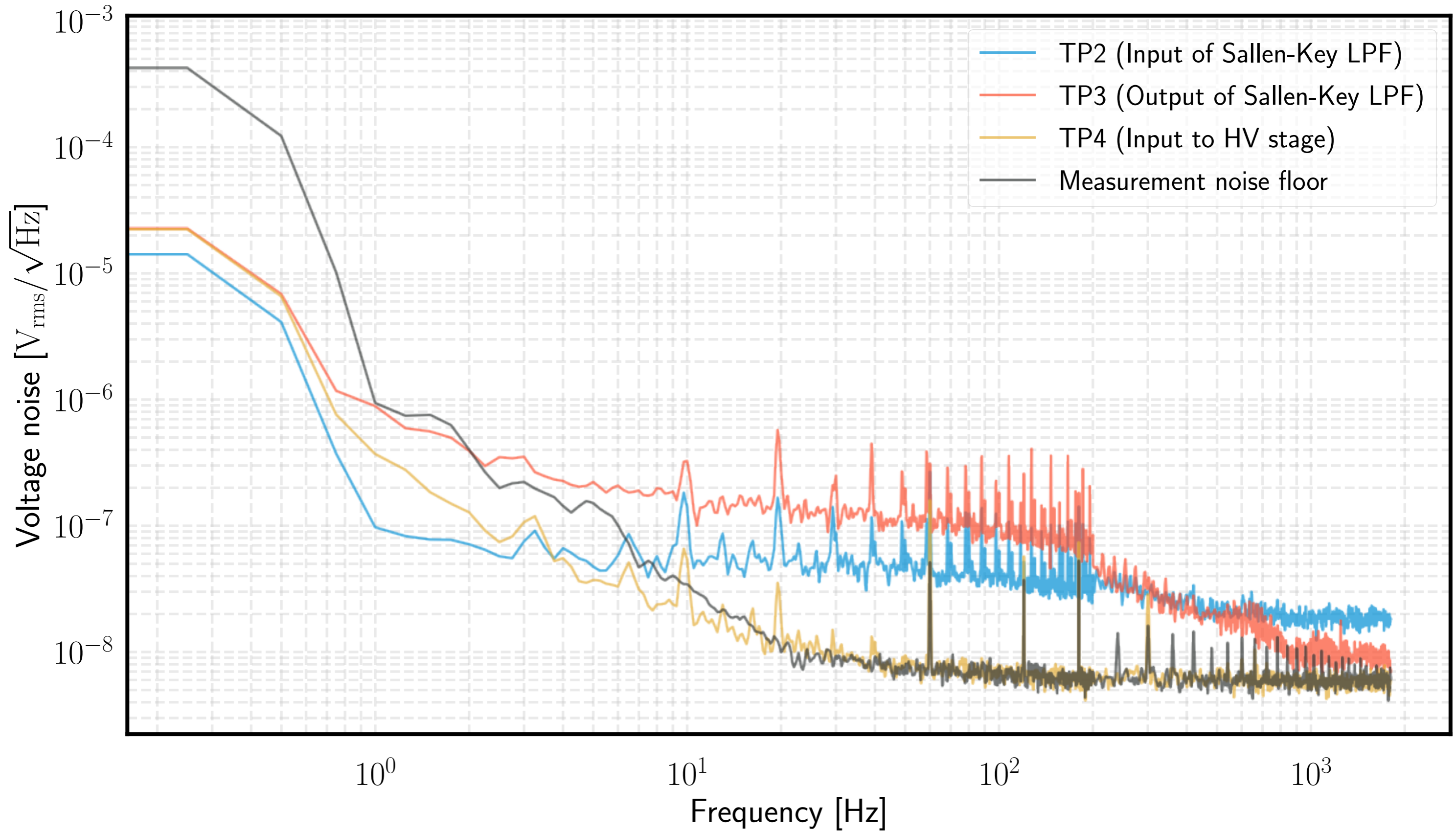
Noise at various points in Low-Voltage part of circuit
