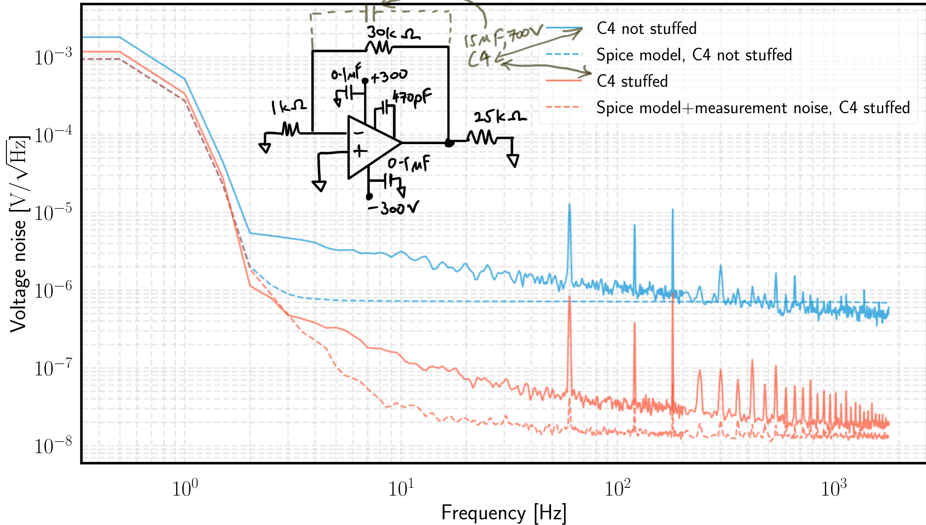
Characterization of HV stage, isolated from Acromag filtering stage (R3 removed)
