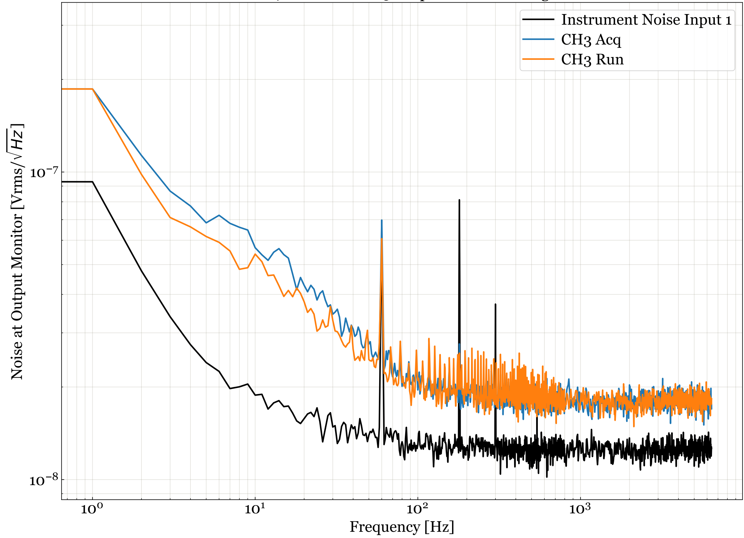
D11000687 S2100028 CH3 Output Monitor Voltage Noise
