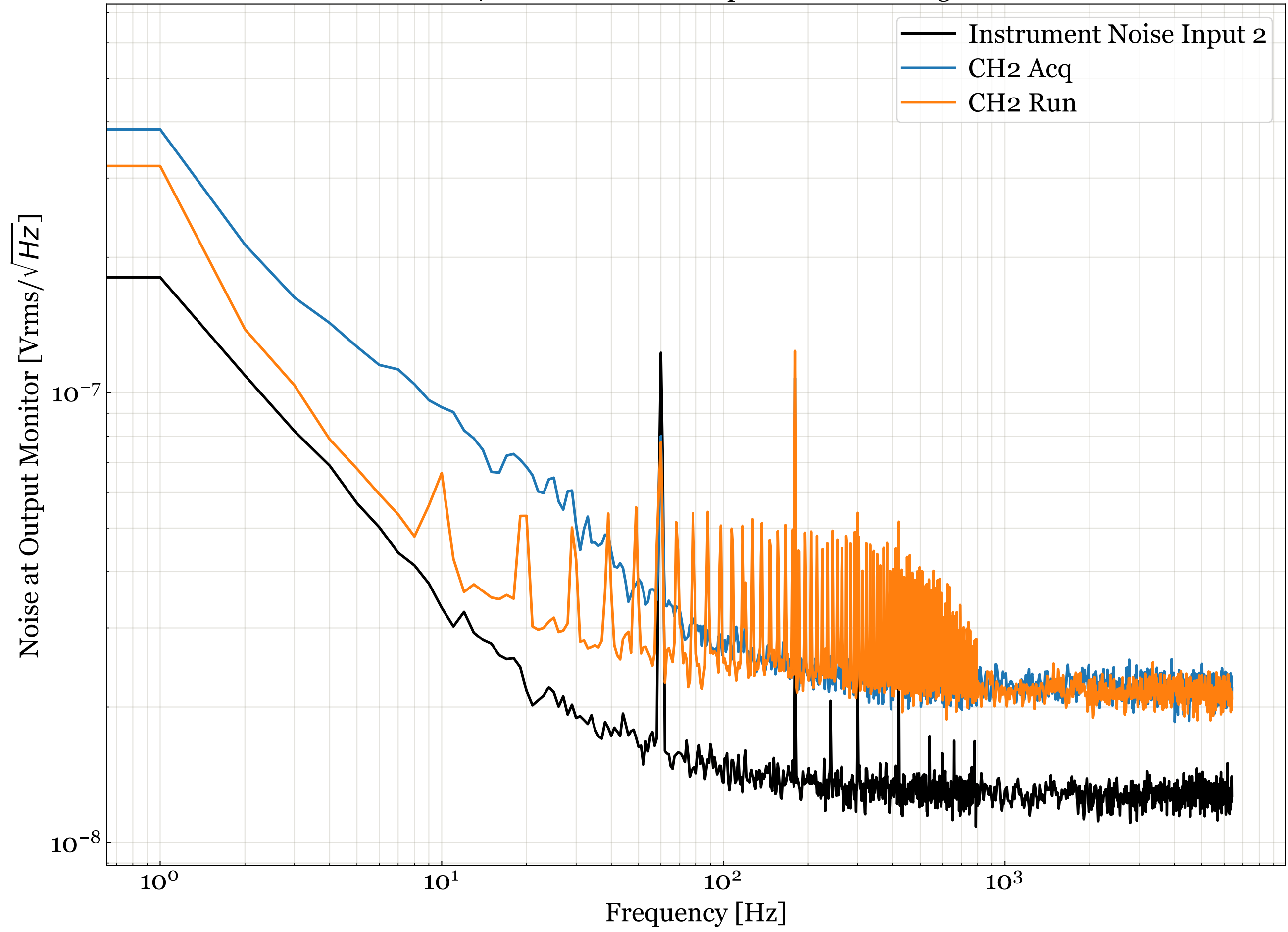
D11000687 S2100028 CH2 Output Monitor Voltage Noise
