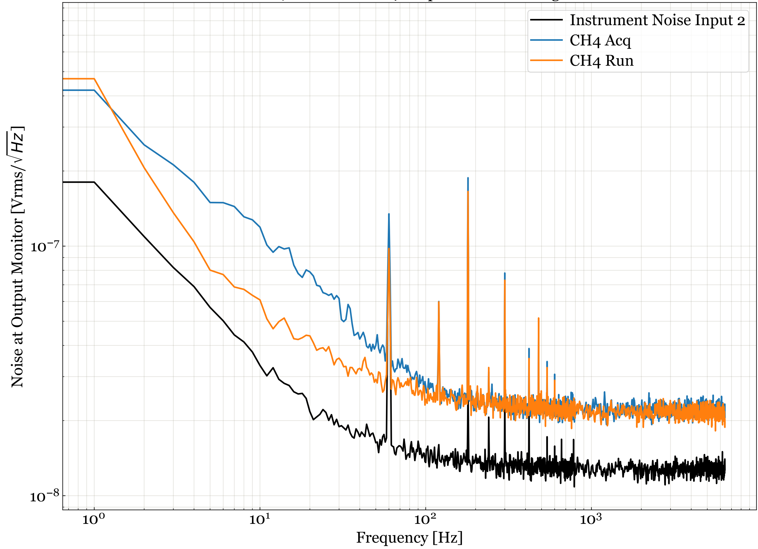
D11000687 S2100028 CH4 Output Monitor Voltage Noise
