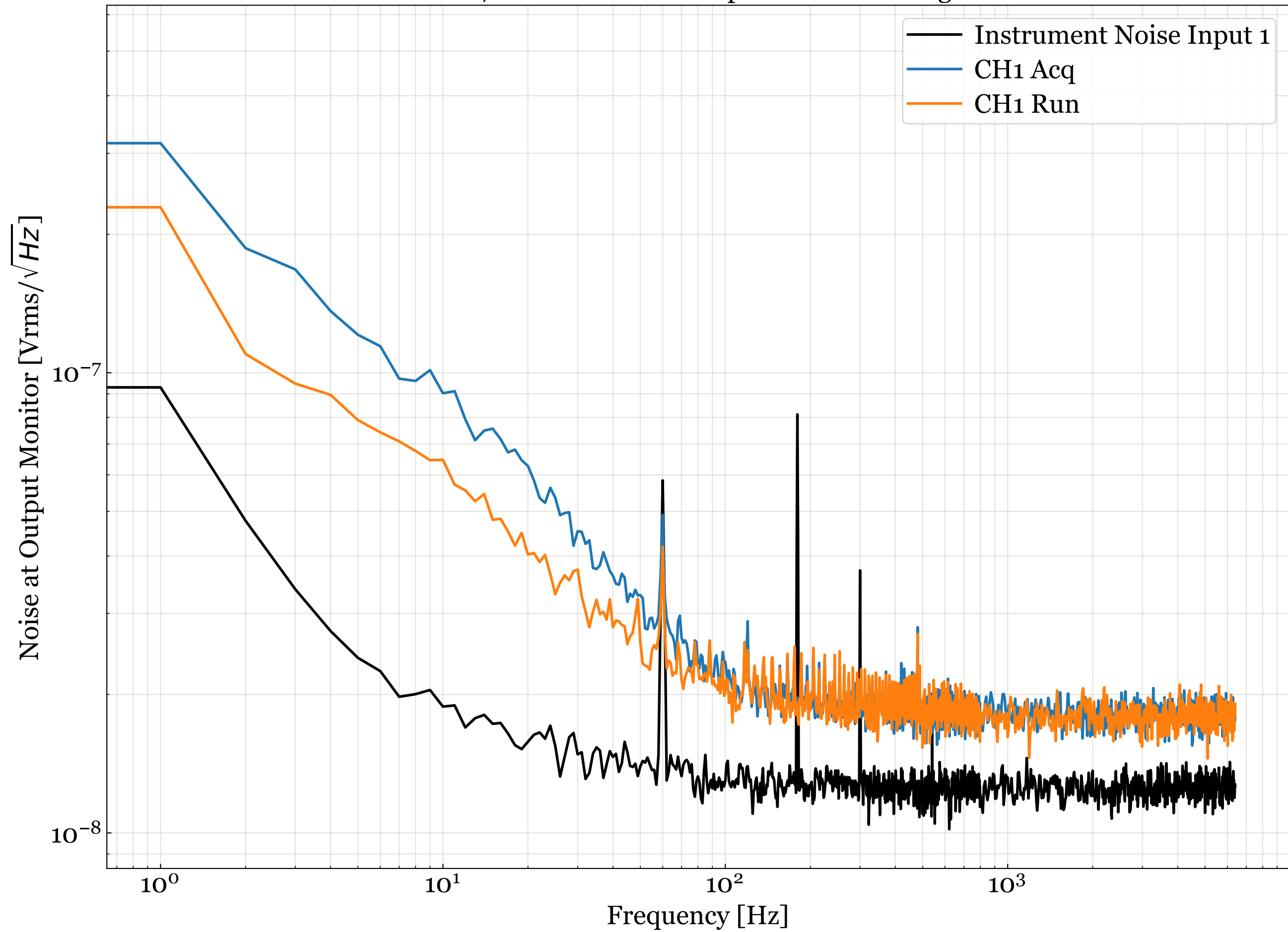
D11000687 S2100028 CH1 Output Monitor Voltage Noise
