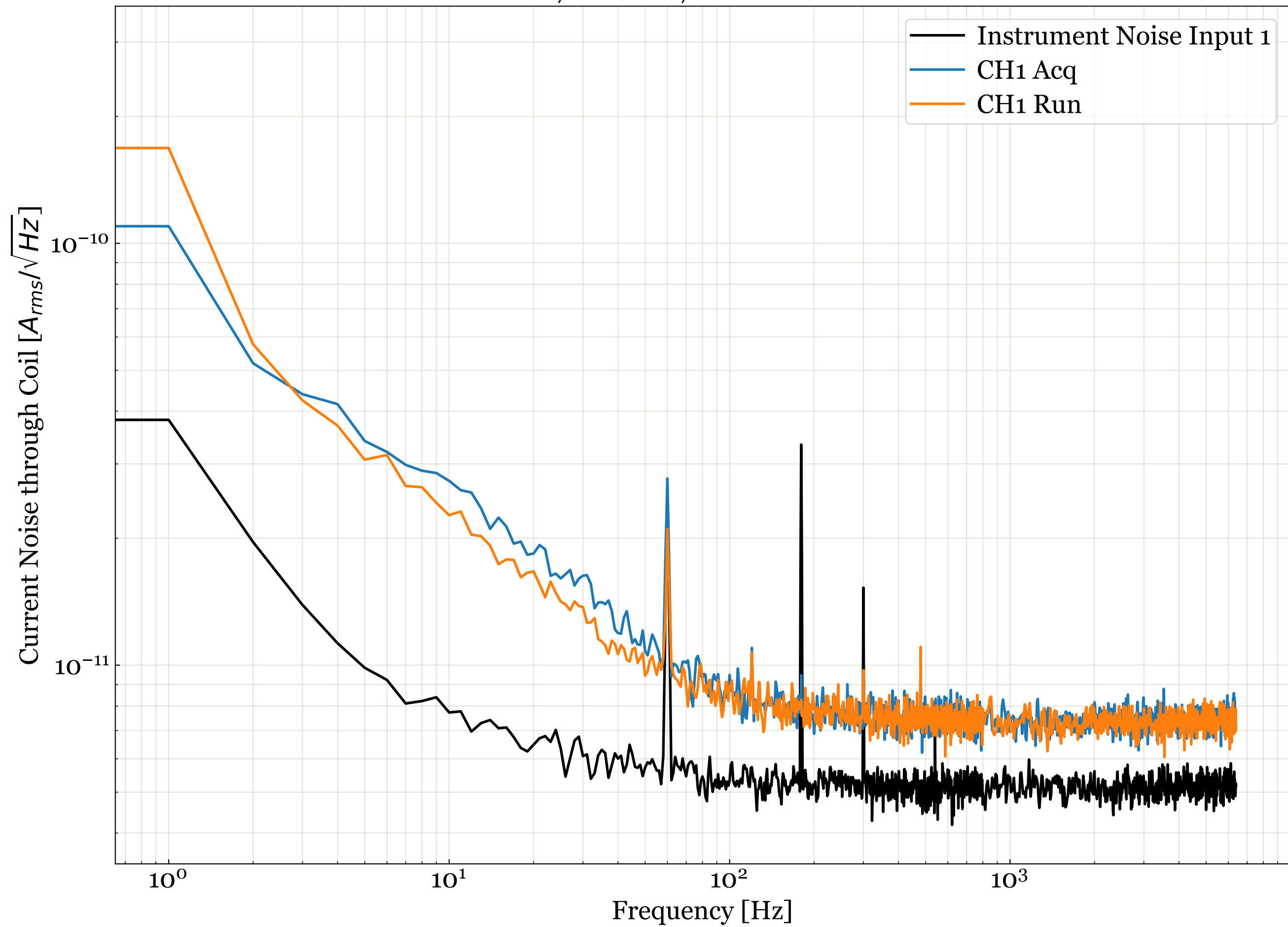
D11000687 S2100027 CH1 Coil Current Noise
