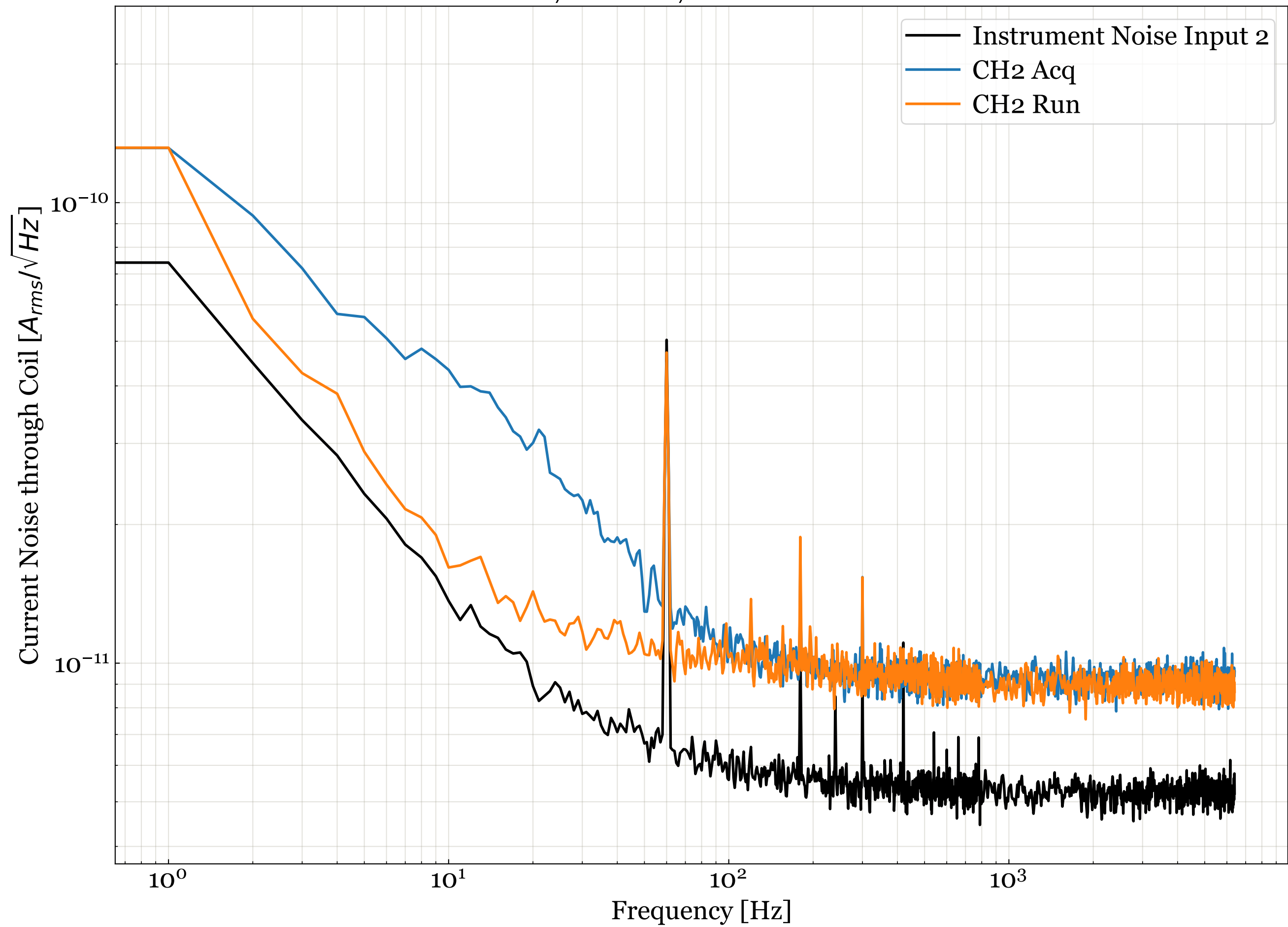
D11000687 S2100027 CH2 Coil Current Noise
