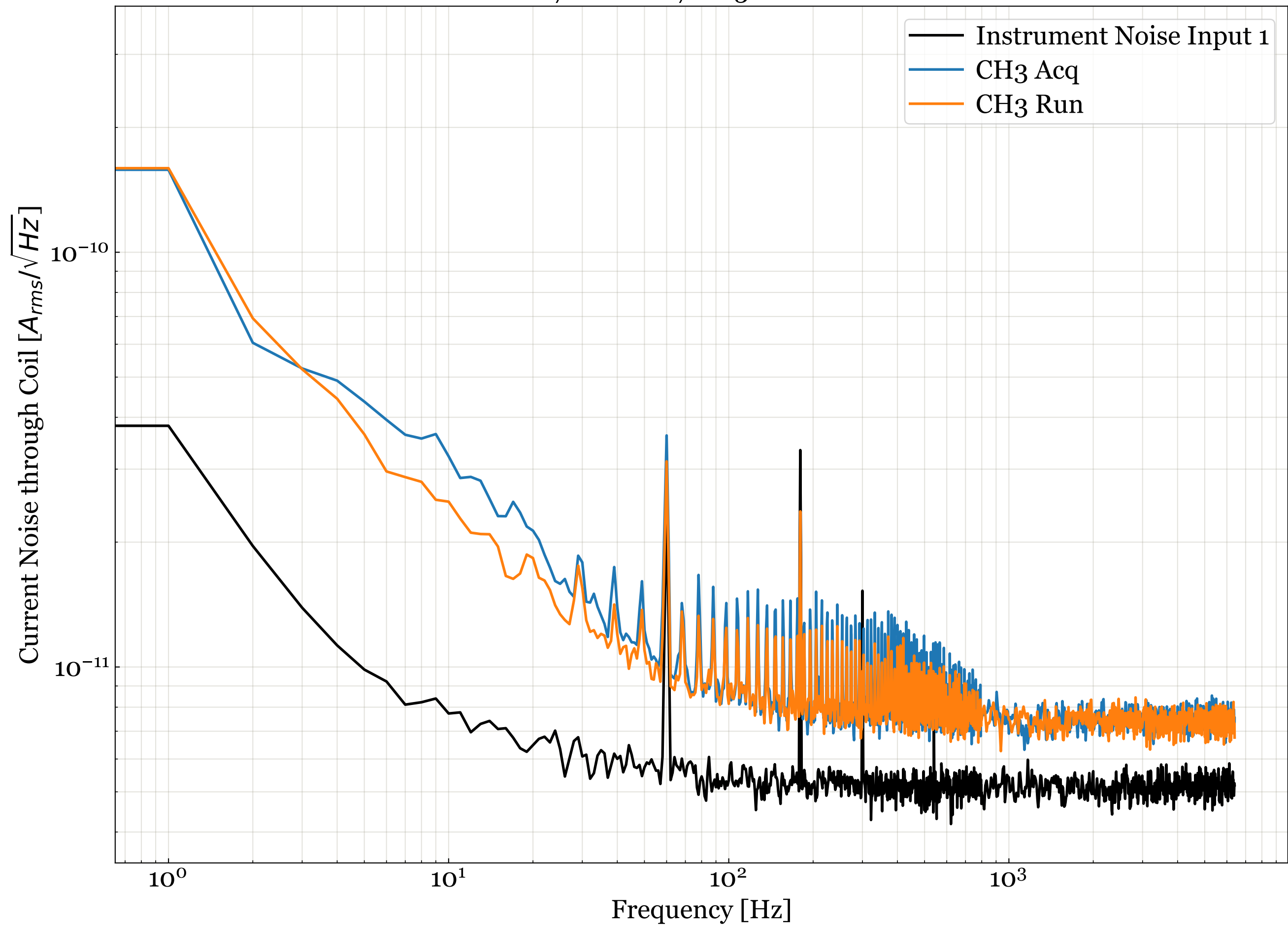
D11000687 S2100027 CH3 Coil Current Noise
