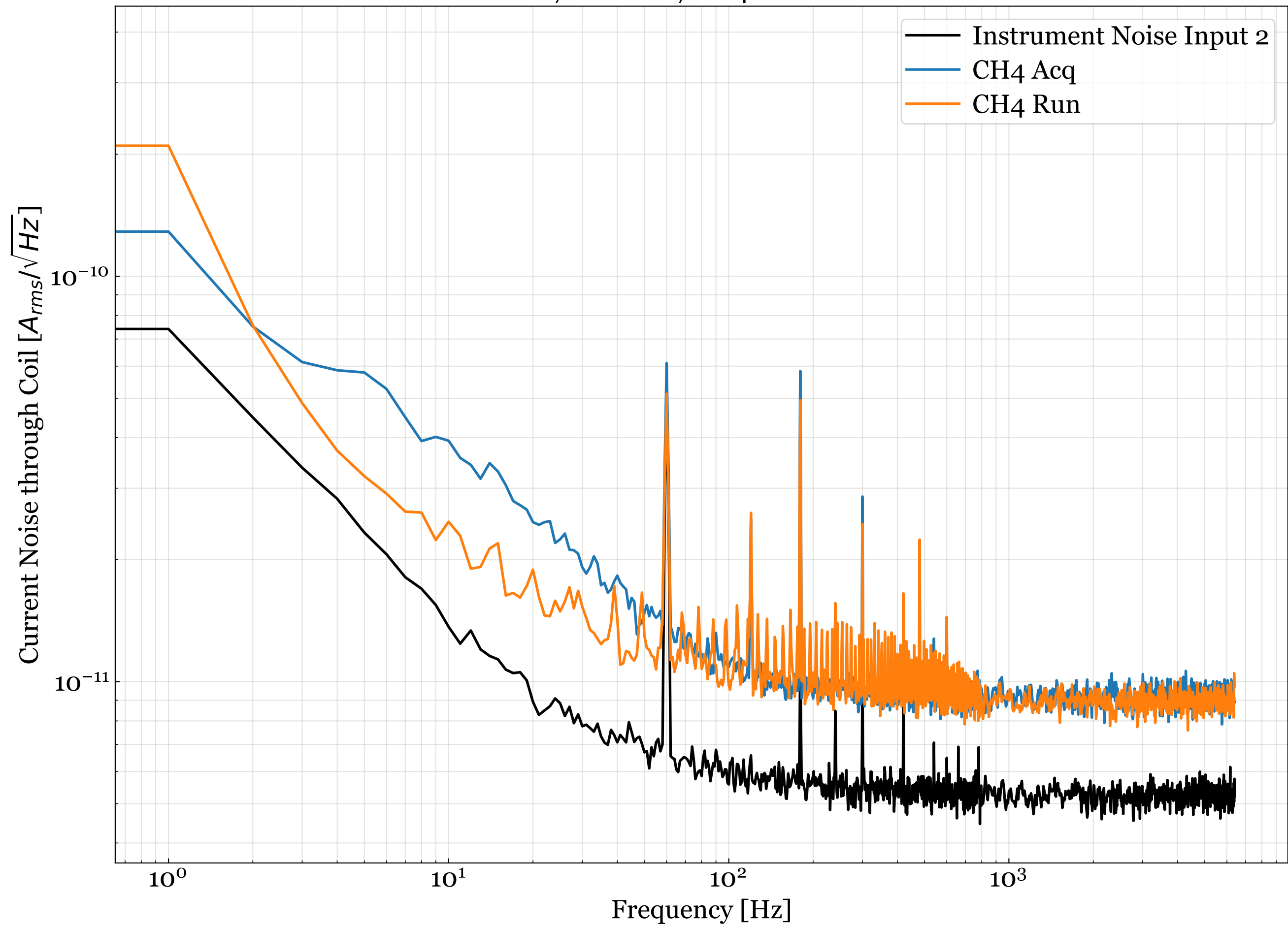
D11000687 S2100027 CH 4 Coil Current Noise
