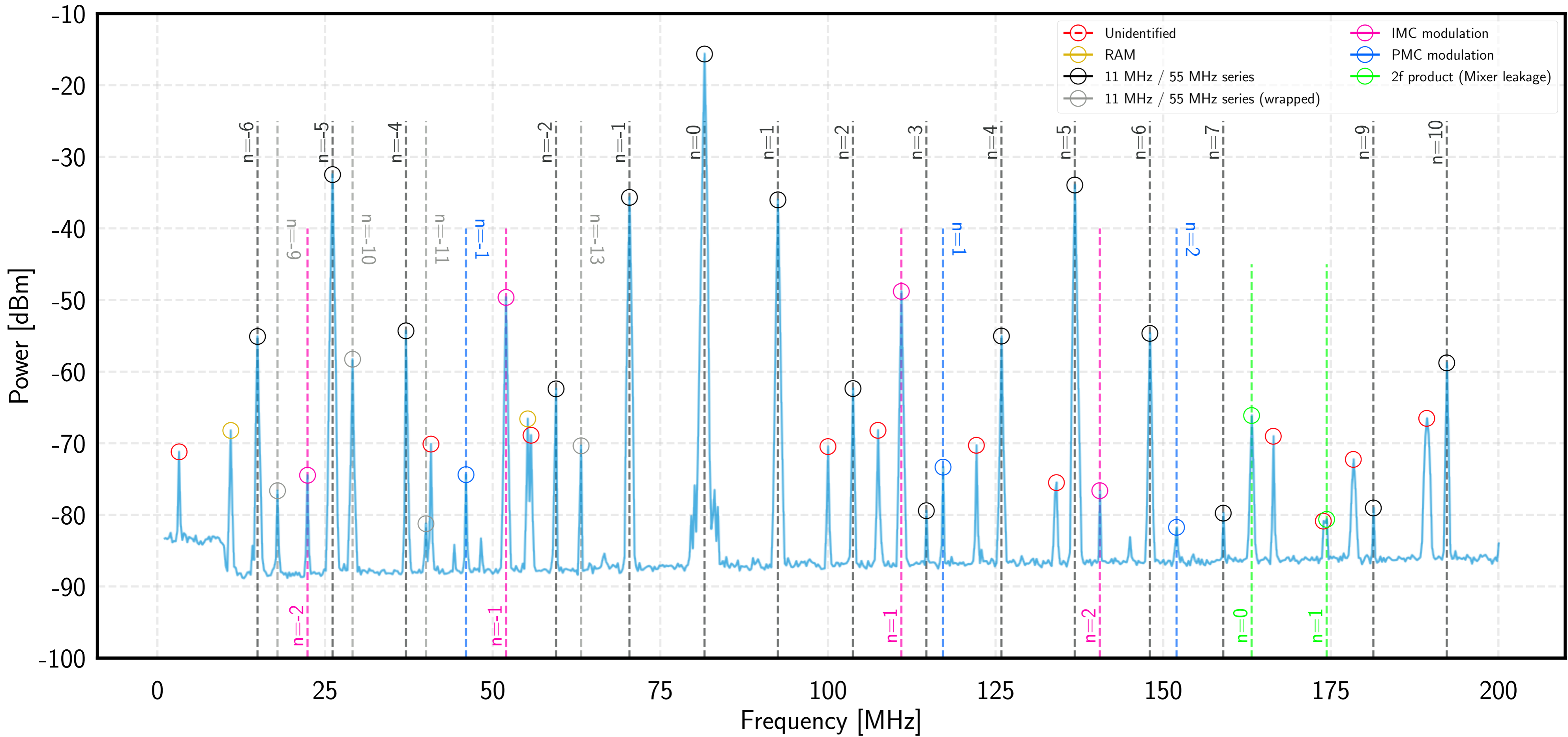
40m PSL beam RF modulation spectrum, Dec 2020
