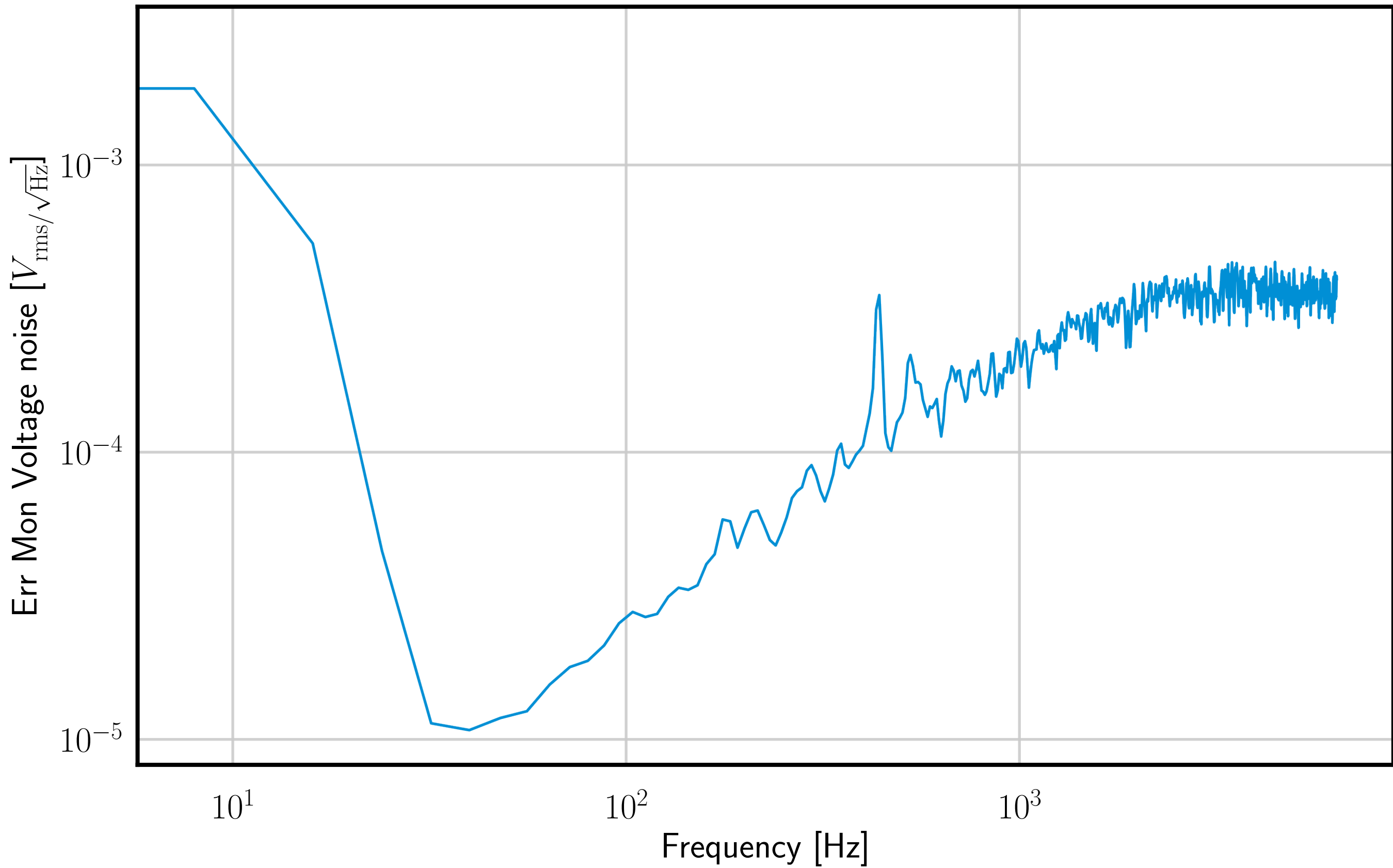
EX uPDH error monitor with AUX laser freq. locked to arm cavity length
