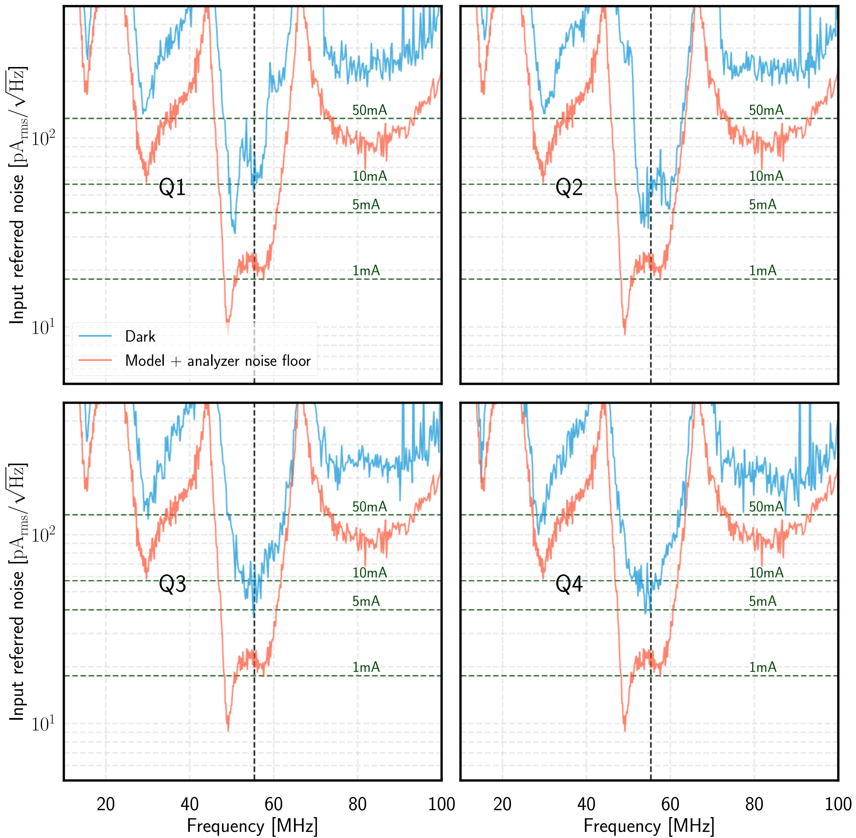
Input referred current noise of WFS quadrants
