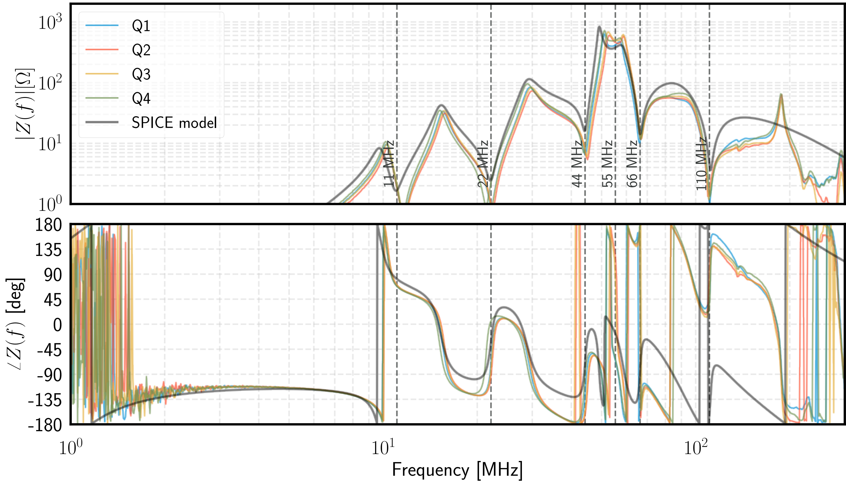
RF High path transimpedance measurement
