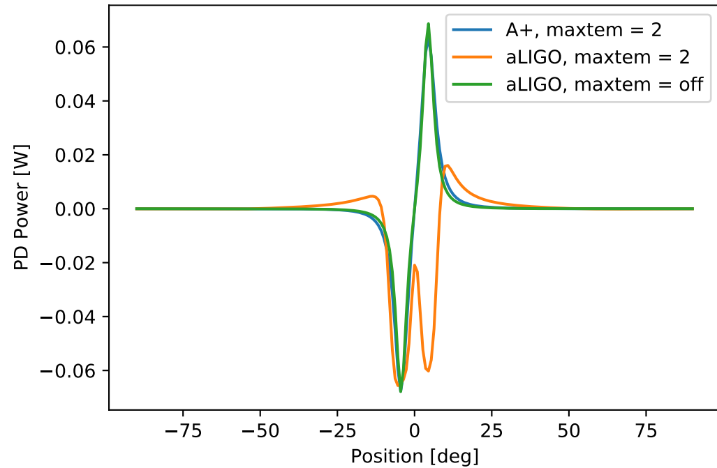
POP_f2_Q (MICH)
