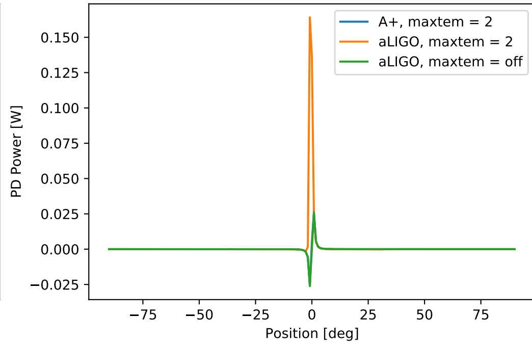
POP_f1_I (PRCL)
