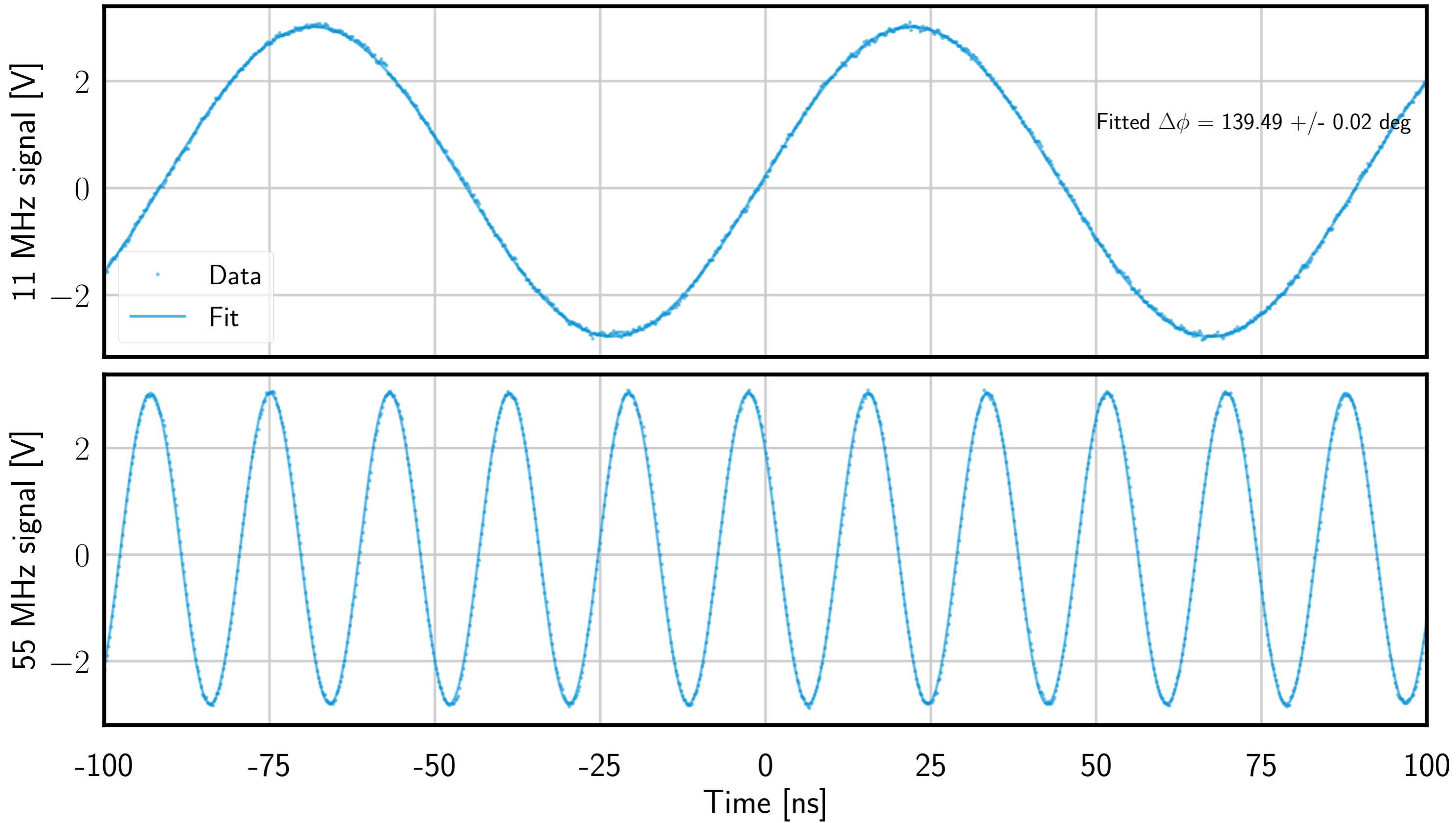
Relative phasing between 11 MHz and 55 MHz signals (EOM path)
