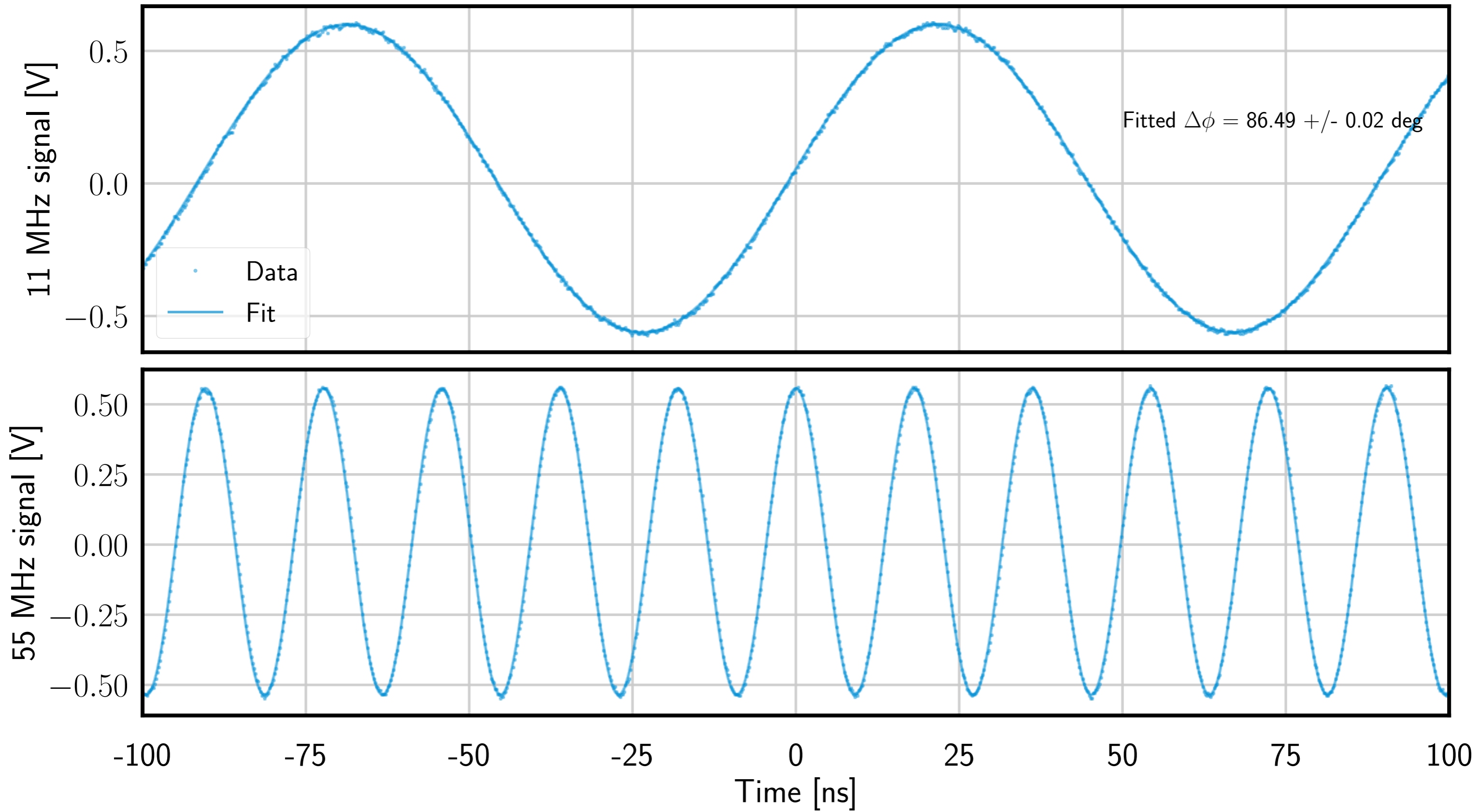
Relative phasing between 11 MHz and 55 MHz signals (Demod path)
