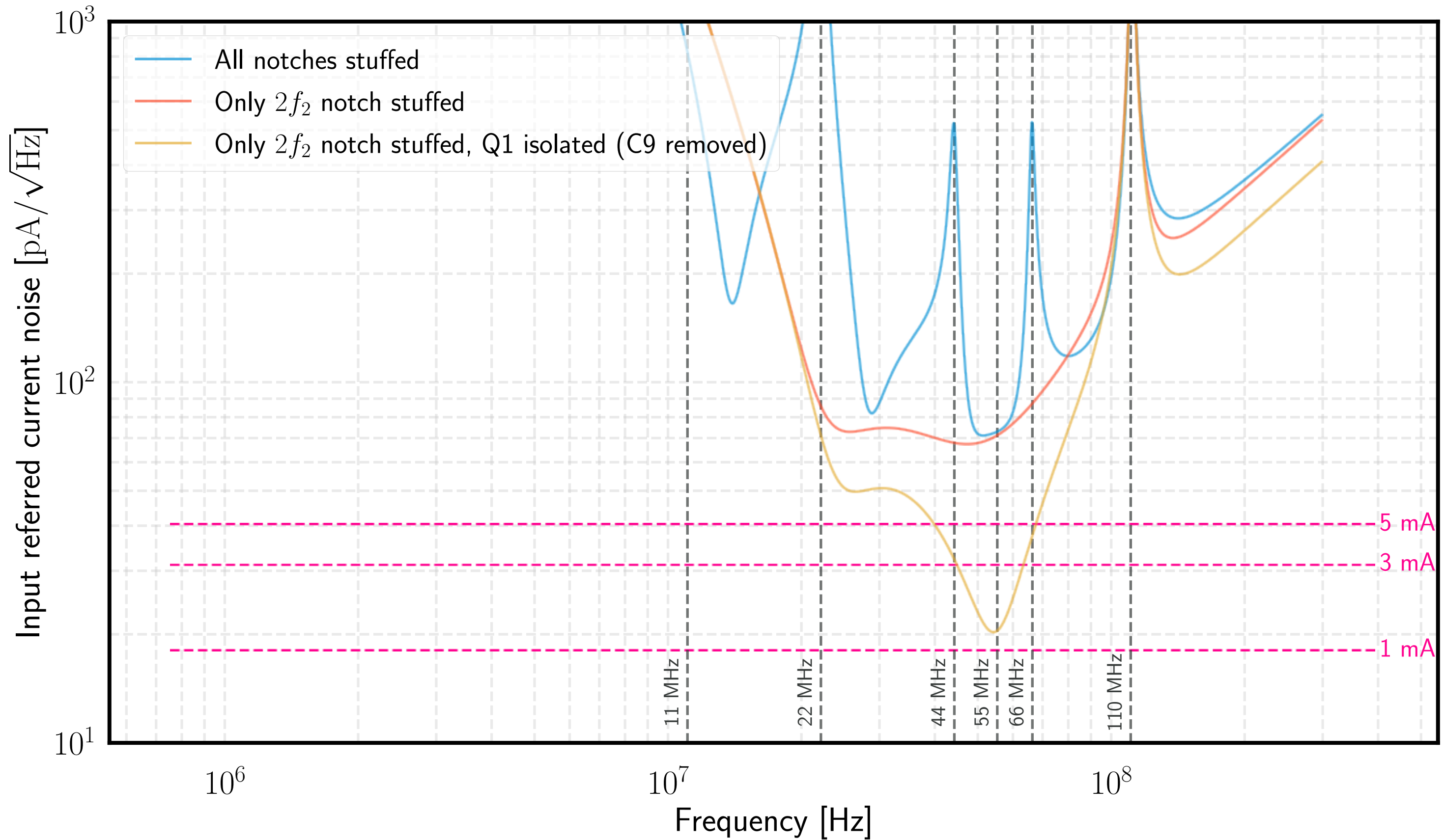
Input referred current noise spectral density for WFS head transimpedance circuit
