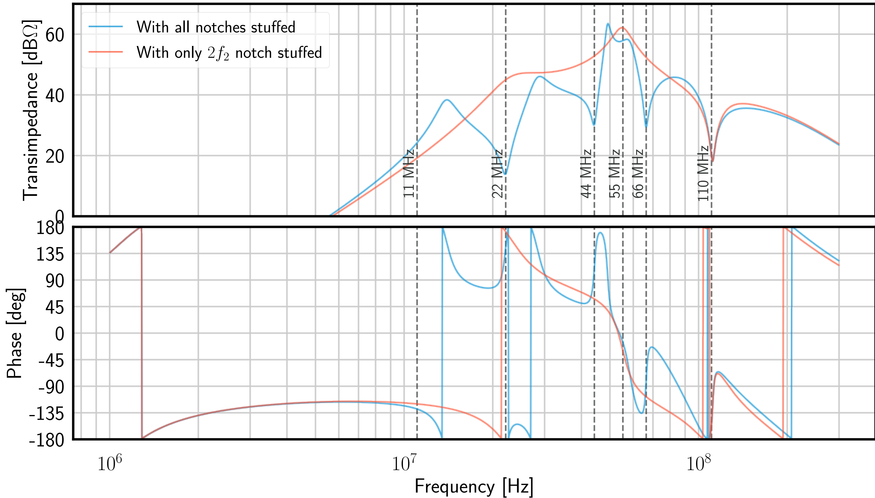
LTspice modelled transfer function for proposed 40m WFS head circuit
