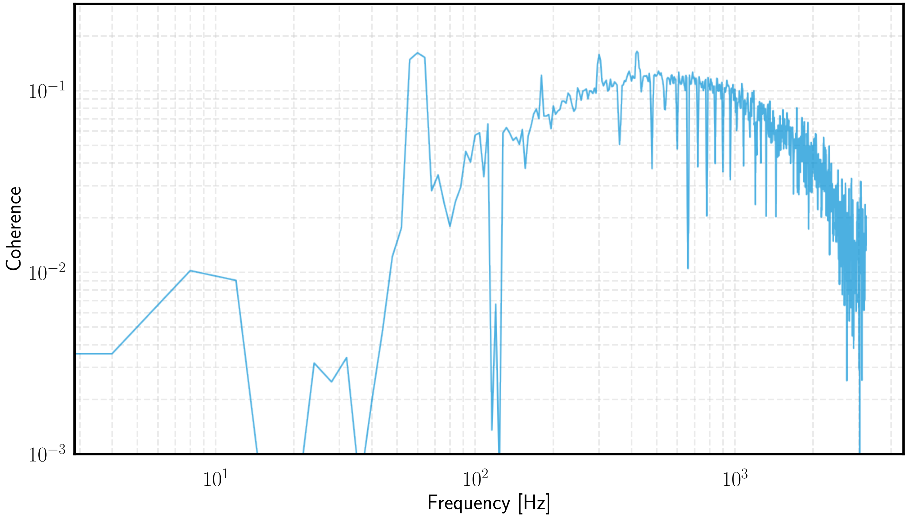
Coherence between positive supply rail and output voltage
