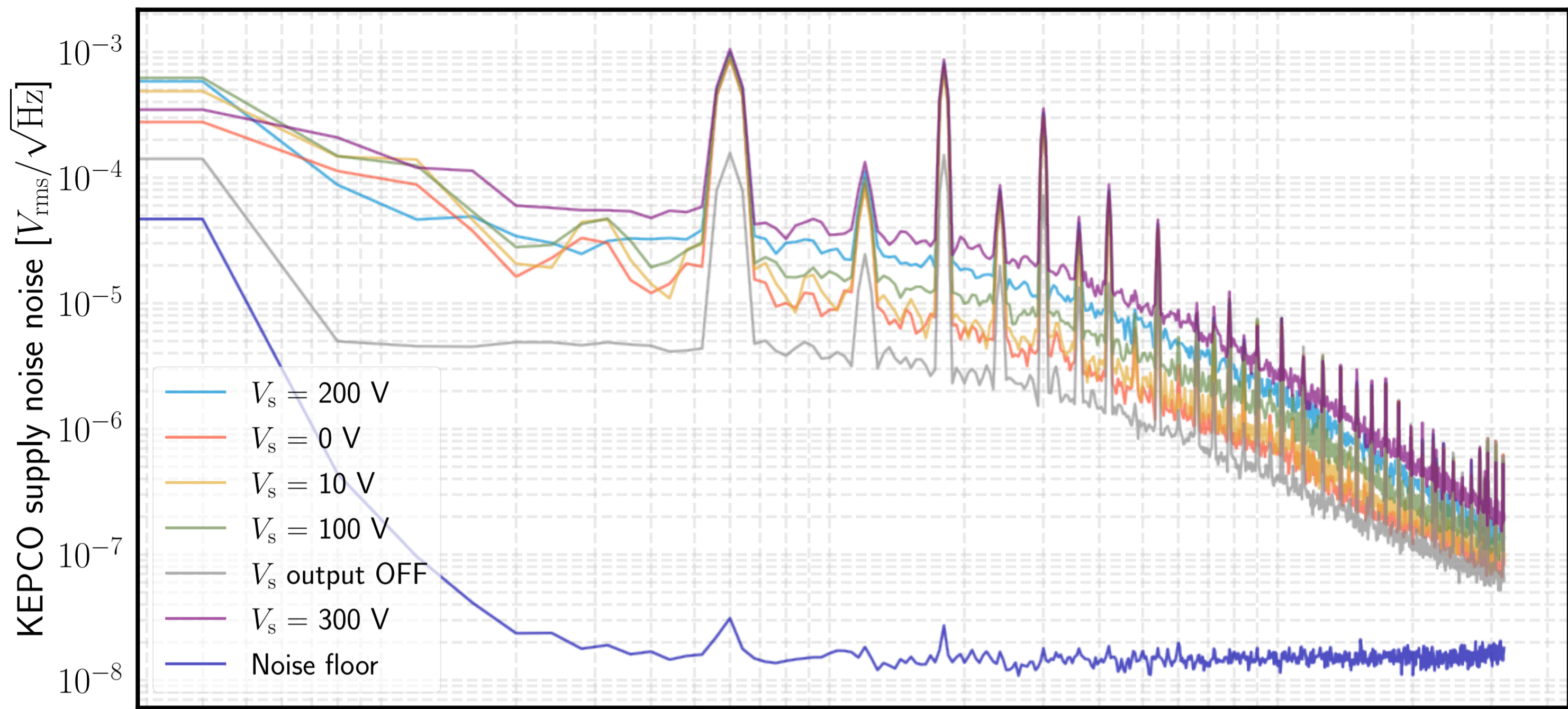
Power supply and HV amp stage noise measurements
