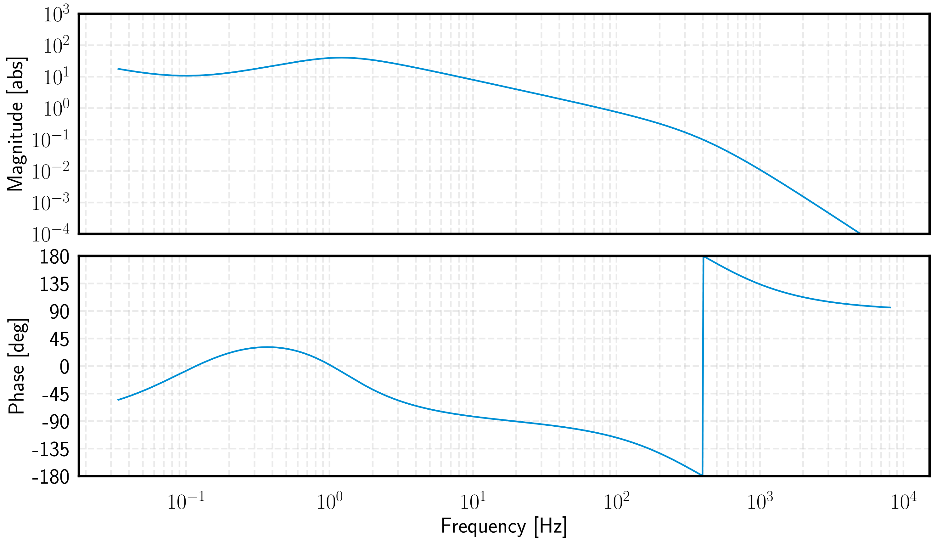
OLTF of proposed loop
