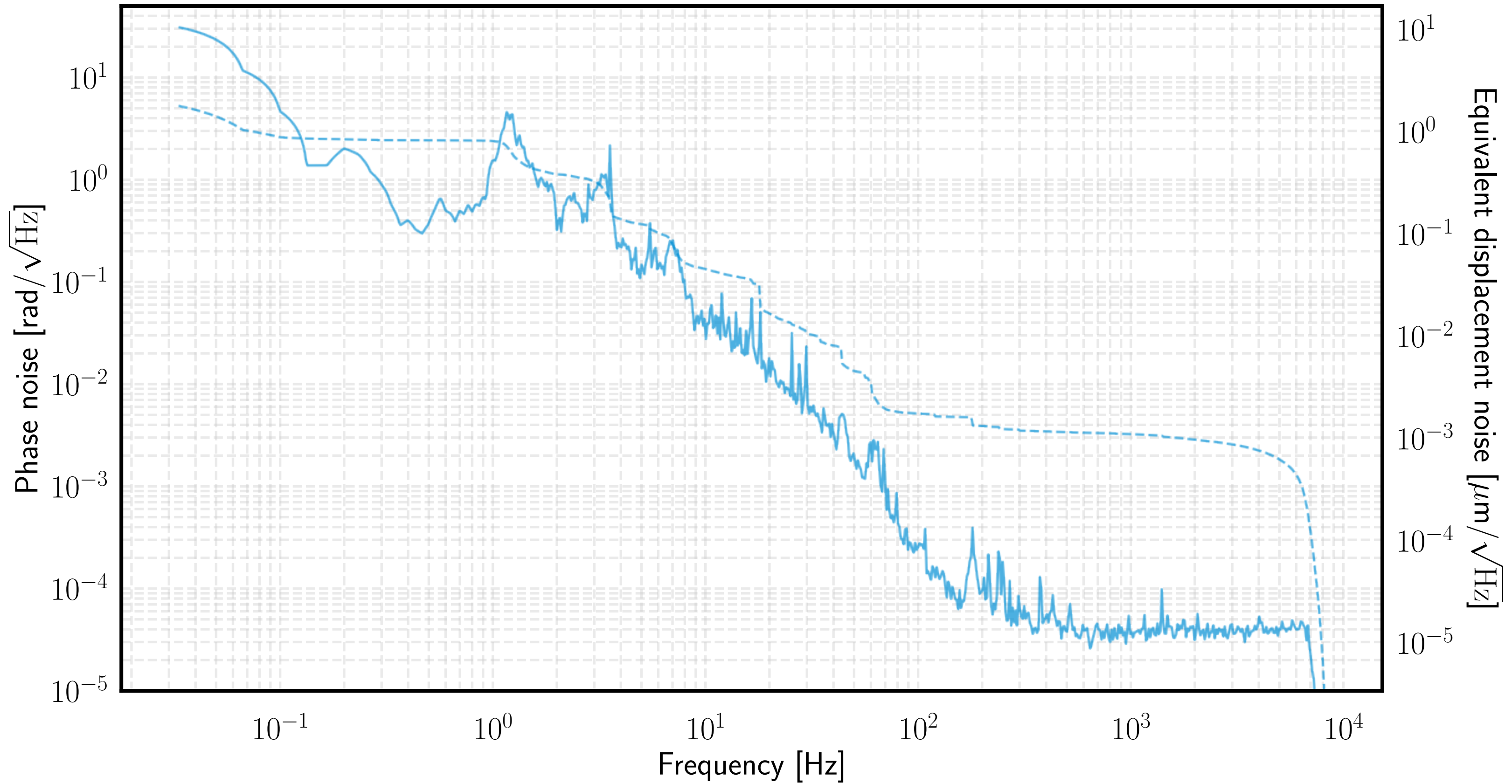
Relative phase noise between LO and signal fields with Michelson locked to dark fringe
