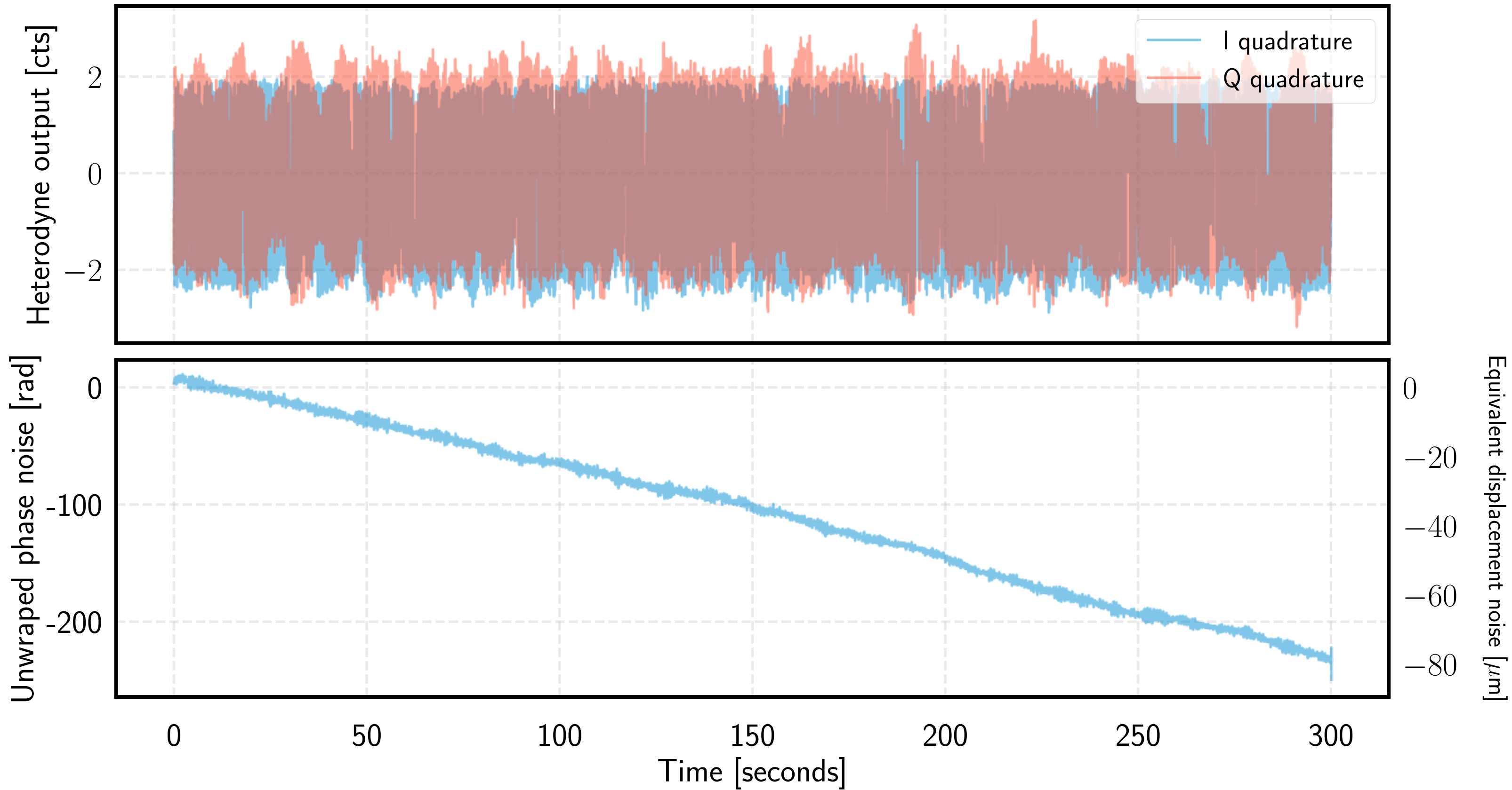
Phase drift between LO and AS fields (simple Michelson locked to dark fringe)
