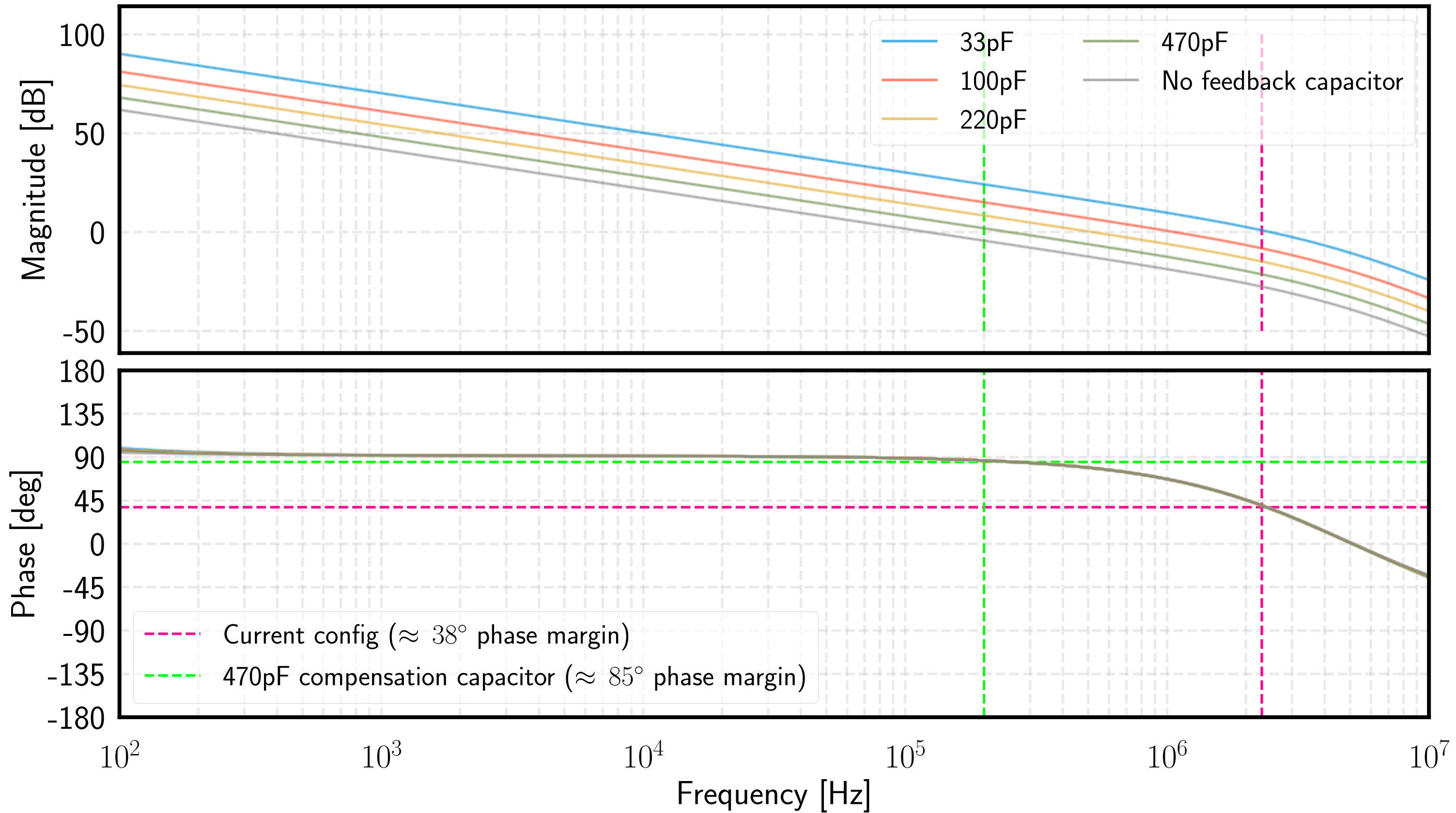
Models of Open-loop gain of PA95 stage of D1900163
