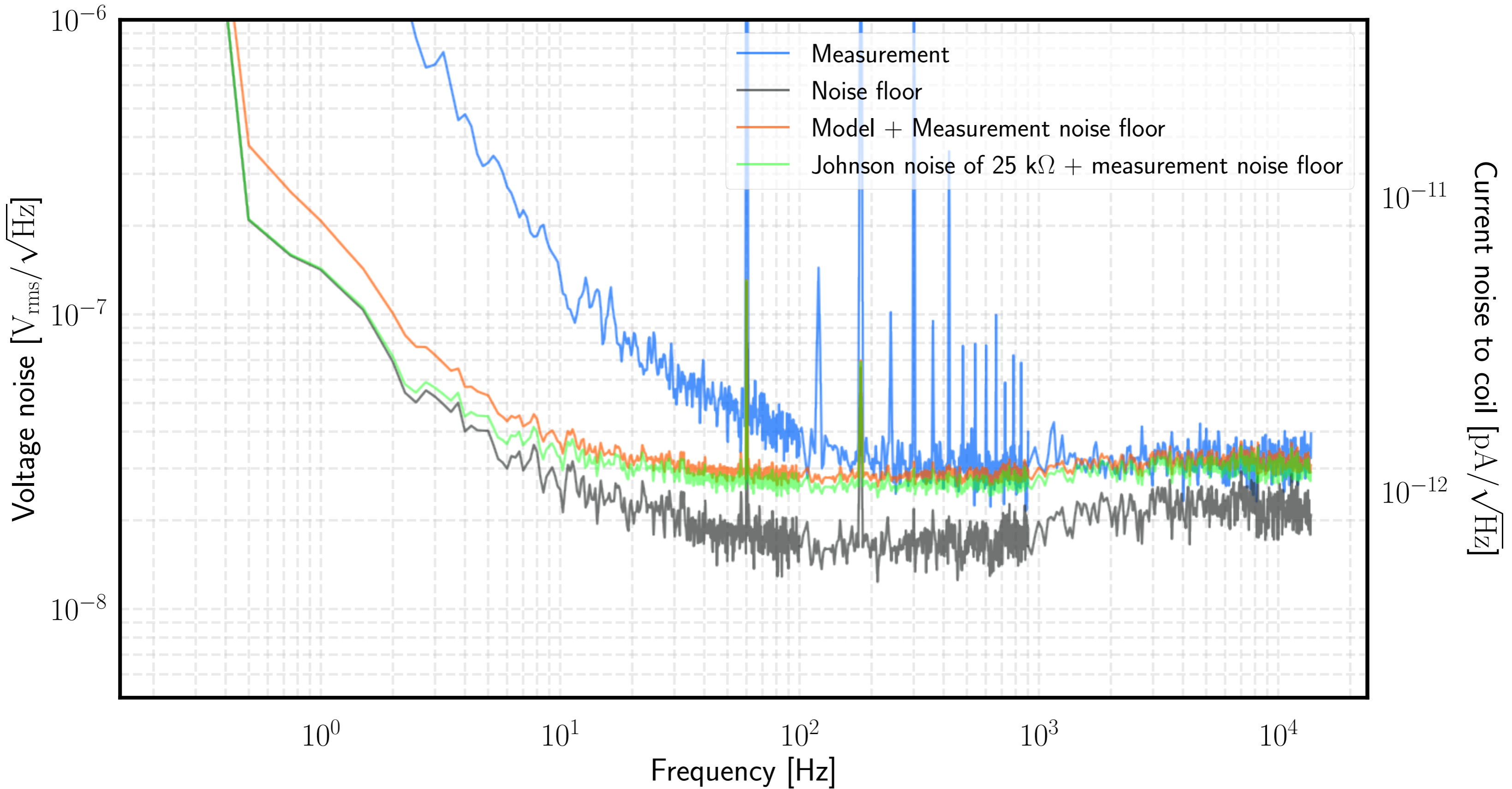
HV coil driver circuit noise measurement
