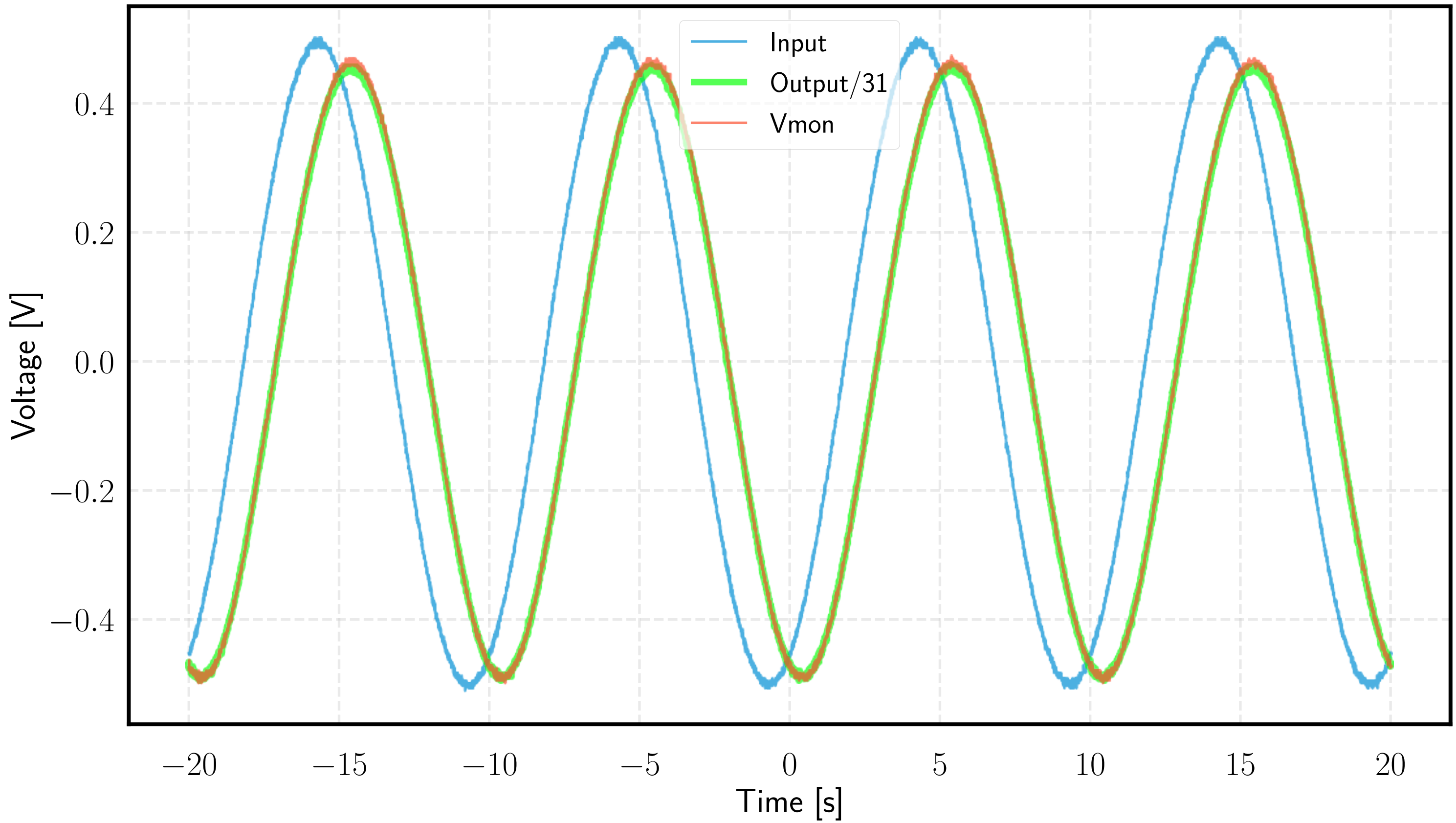
HV coil driver - input driven with 0.1 Hz sine wave
