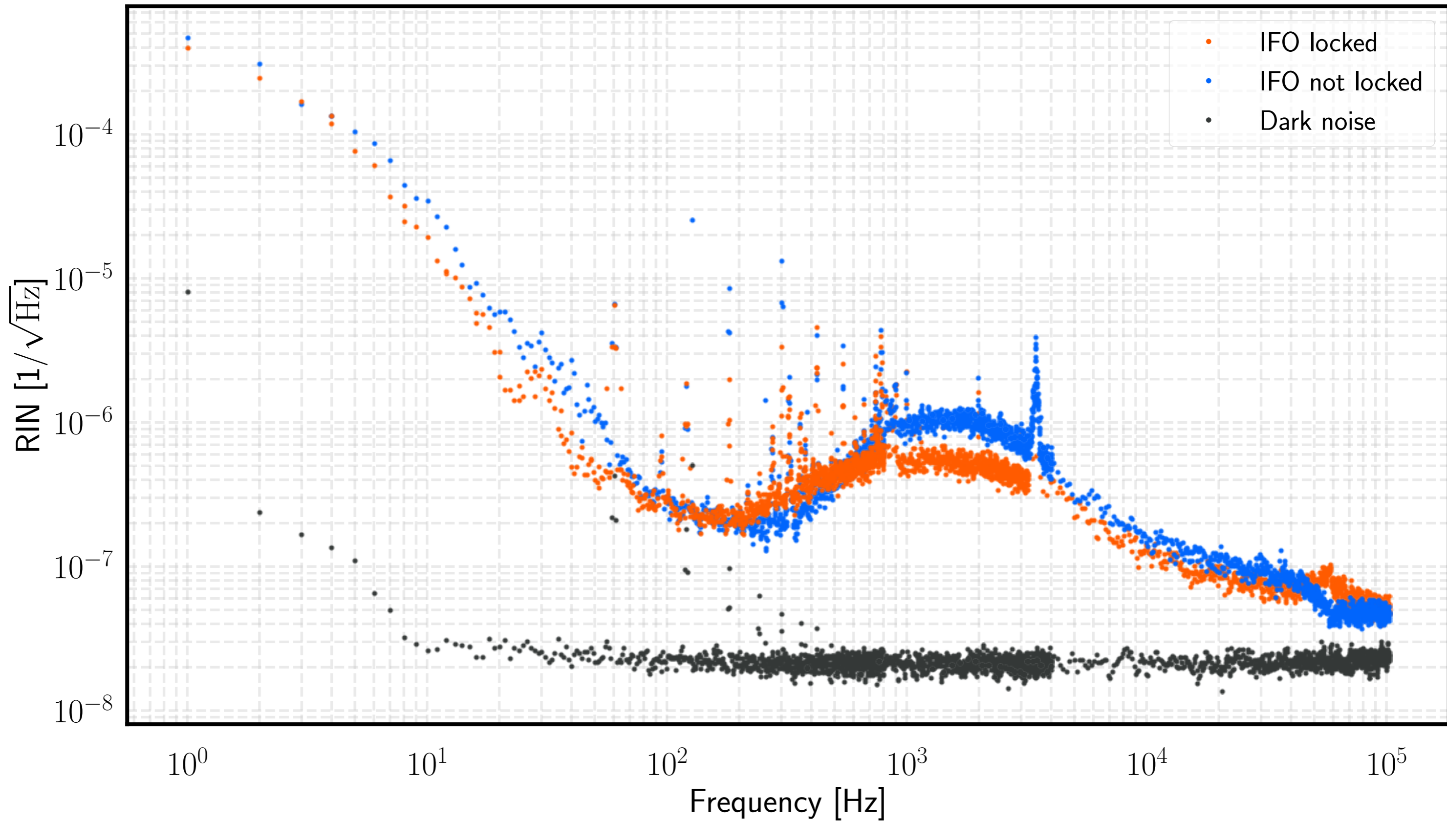
Local oscillator pickoff RIN, with PRFPMI [PDA 520 DC value = 3.75 V]
