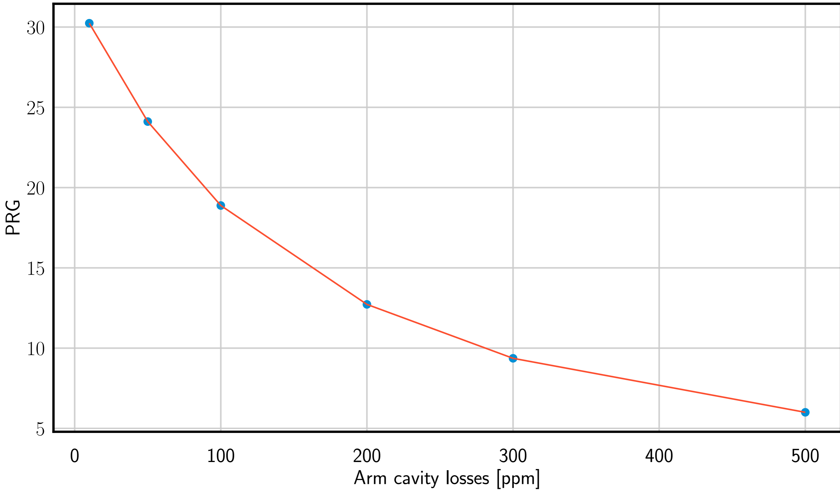
PRG dependence on arm cavity losses, assuming \eta_{\text{PRC}} = 2.0\%
